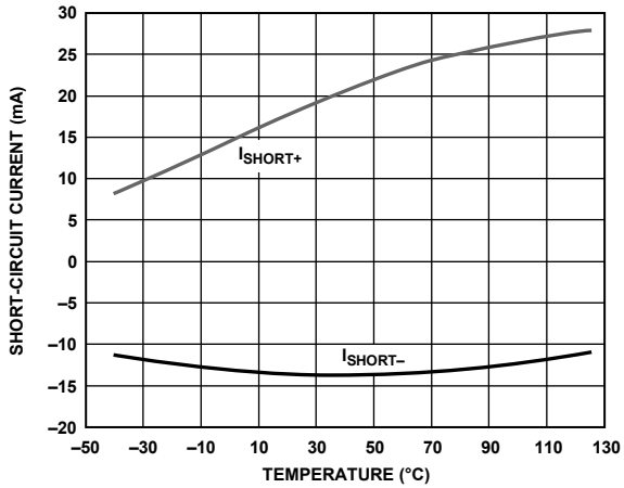
Figure 25. Short-Circuit Current Per Channel vs. Temperature
