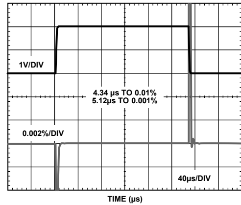
Figure 29. Large-Signal Pulse Response and Settling Time, 2 V Step, V_S = 2.7 V
