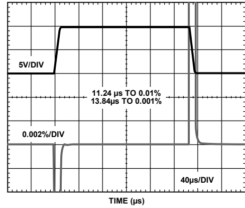
Figure 28. Large-Signal Pulse Response and Settling Time, 10 V Step, V_S = \pm 15 V
