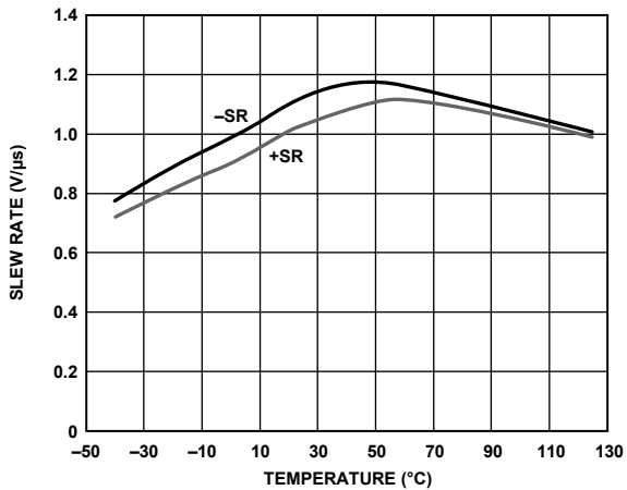
Figure 26. Slew Rate vs. Temperature, V_{IN} = 20 V p-p , 1 kHz
