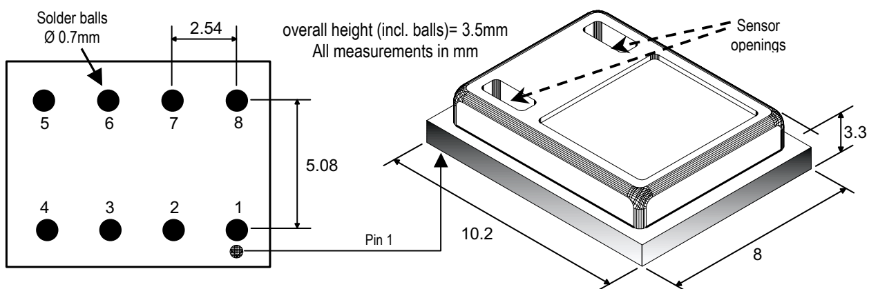
Figure 7 AH31 Mounting Information, bottom and side view.
