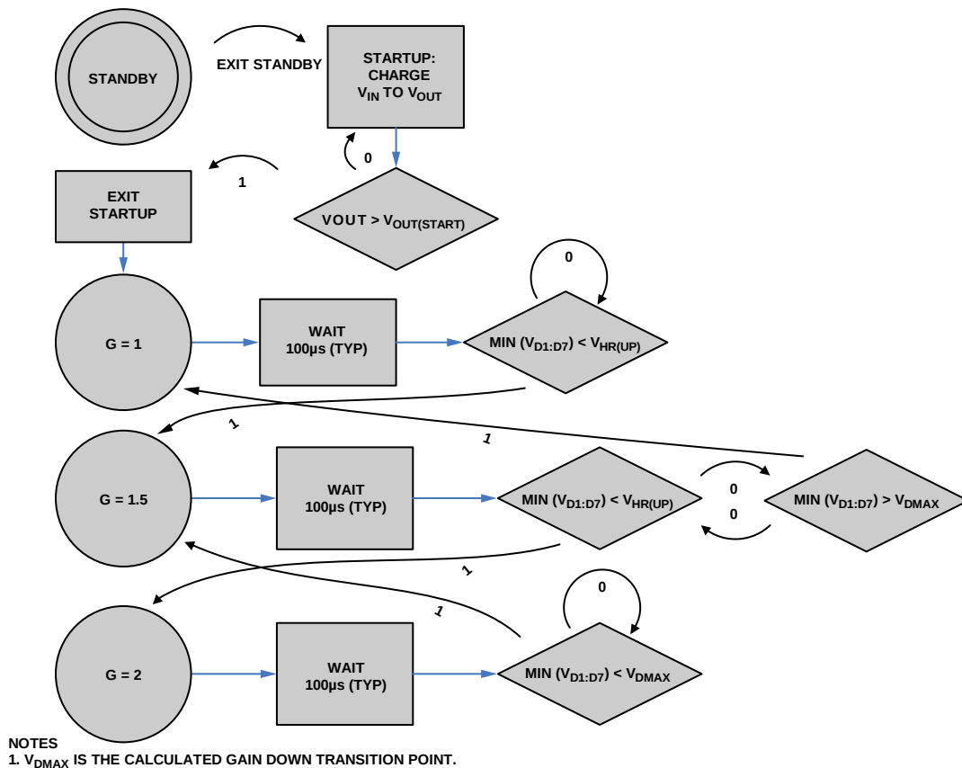
Figure 26. State Diagram for Automatic Gain Selection Rev. A | Page 12 of 40
