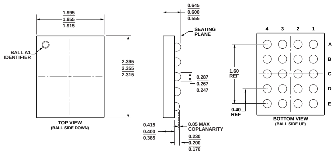
Figure 46. 20-Ball Wafer Level Chip Scale Package [WLCSP] (CB-20-6) Dimensions shown in millimeters
