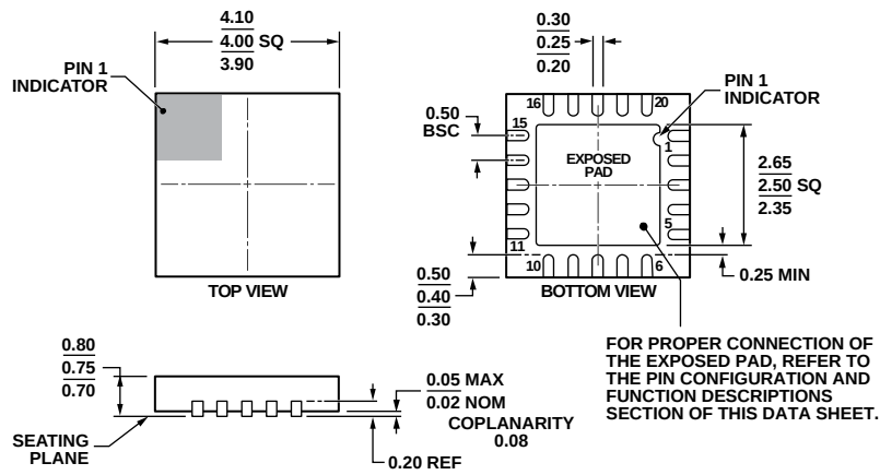
Figure 44. 20-Lead Lead Frame Chip Scale Package [LFCSP_WQ] 4 mm × 4 mm Body, Very Thin Quad (CP-20-10) Dimensions shown in millimeters
