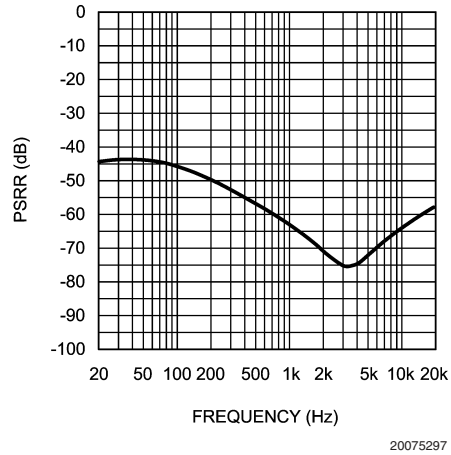
PSRR vs Frequency V_{DD} = 5V, R_L = 32\Omega, V_{RIPPLE} = 100mV_{pp} Inputs Terminated
