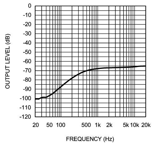
Crosstalk vs Frequency V_{DD} = 5V, R_L = 8\Omega
