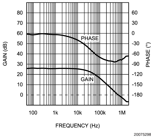
Open Loop Frequency Response V_{DD} = 5V, R_L = 8\Omega
