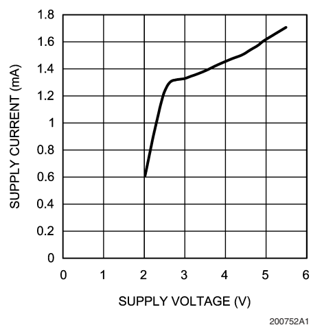
Supply Current vs Supply Voltage (no Load)
