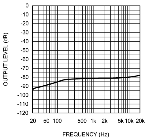
Crosstalk vs Frequency V_{DD} = 5V, R_L = 32\Omega
