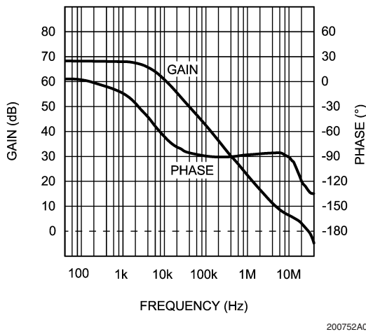
Open Loop Frequency Response V_{DD} = 5V, R_L = 5k\Omega
