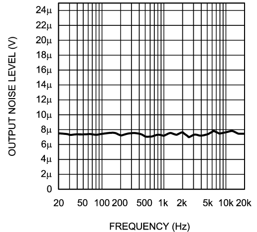
Output Noise vs Frequency V_{DD} = 5V, R_L = 32\Omega
