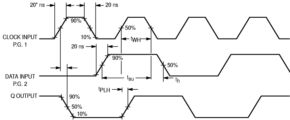
Figure 2. AC Test Circuit and Timing Diagram (Clock to Output)
