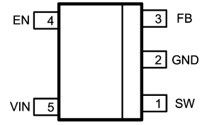
5-Pin SOT-23
