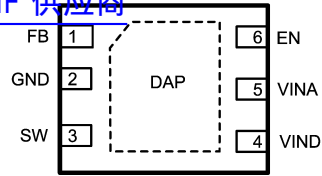
6-Pin LLP
