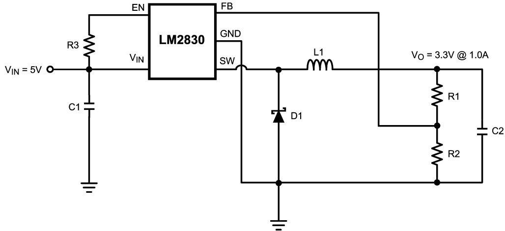
FIGURE 9. LM2830Z (3MHz): V_{IN} = 5V , V_O = 3.3V @ 1.0A
