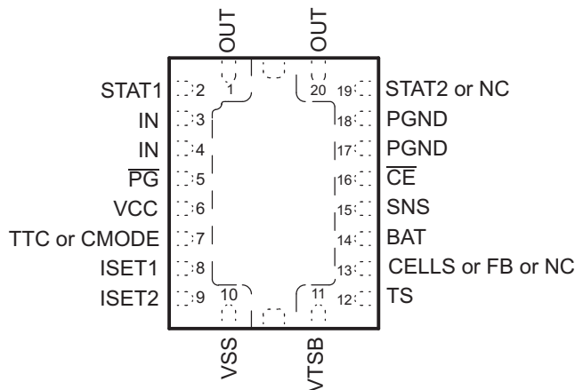
RHL PACKAGE (TOP VIEW) (bq24100, 03, 03A, 05, 08, 09, 13, 13A, 15)
