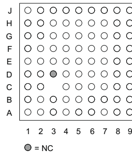
Figure 2-1. Pin Assignments (not to scale)
