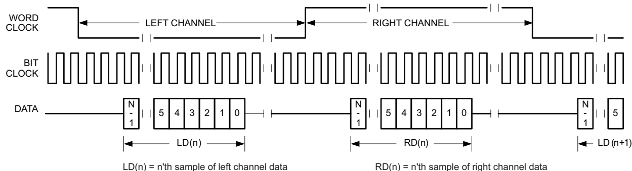
Figure 5-40. Timing Diagram for I²S Mode With Offset = 2
