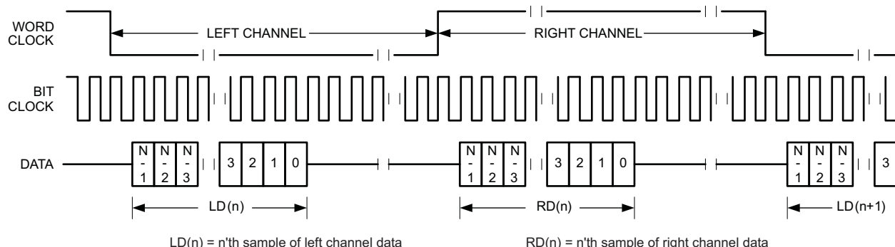
Figure 5-41. Timing Diagram for I²S Mode With Offset = 0 and Bit Clock Invert
