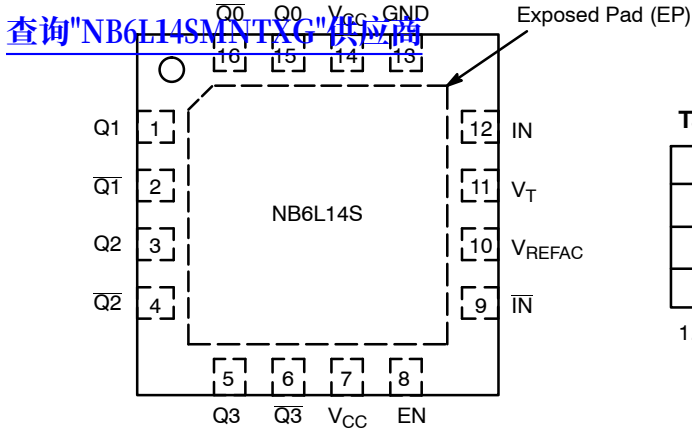
Figure 3. NB6L14S Pinout, 16-pin QFN (Top View)
