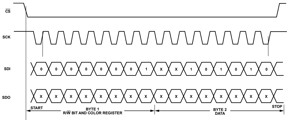
Figure 17. Setting the Green Register to Delay Code 42 Using SPI
