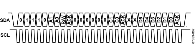
Figure 23. I 2 C 3-Byte Timing Sequence
