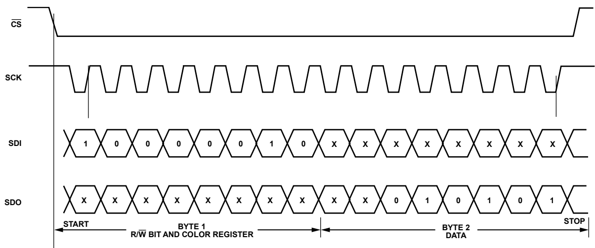
Figure 18. Reading Delay Code 21 from the Blue Register Using SPI
