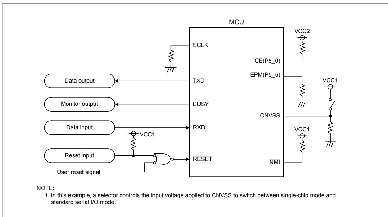
Figure 26.18 Pin Handling in Standard Serial I/O Mode 2
