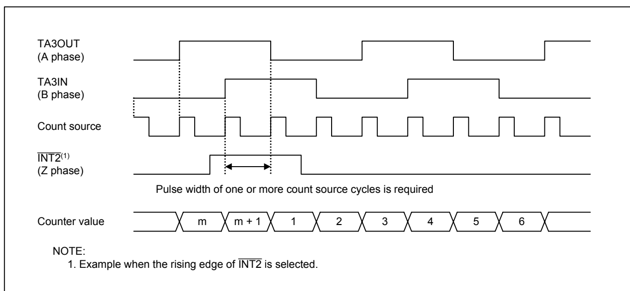
Figure 15.17 Relations between Two-Phase Pulses (A-Phase and B-Phase) and Z-Phase Pulse
