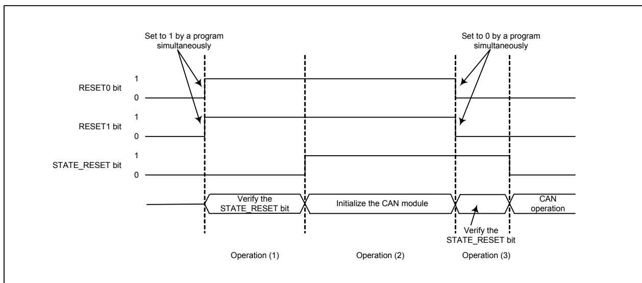
Figure 23.37 Example of CAN Module Initialize Operation
