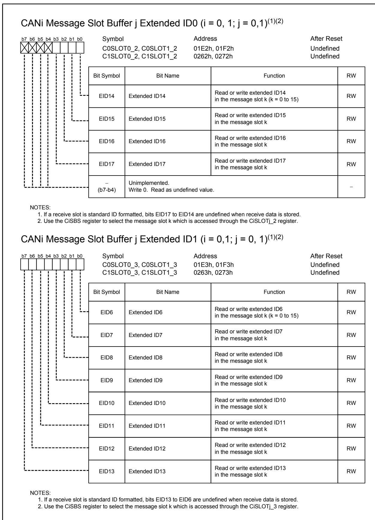
Figure 23.33 C0SLOT0_2, C0SLOT1_2, C1SLOT0_2, and C1SLOT1_2 Registers, C0SLOT0_3, C0SLOT1_3, C1SLOT0_3, and C1SLOT1_3 Registers
