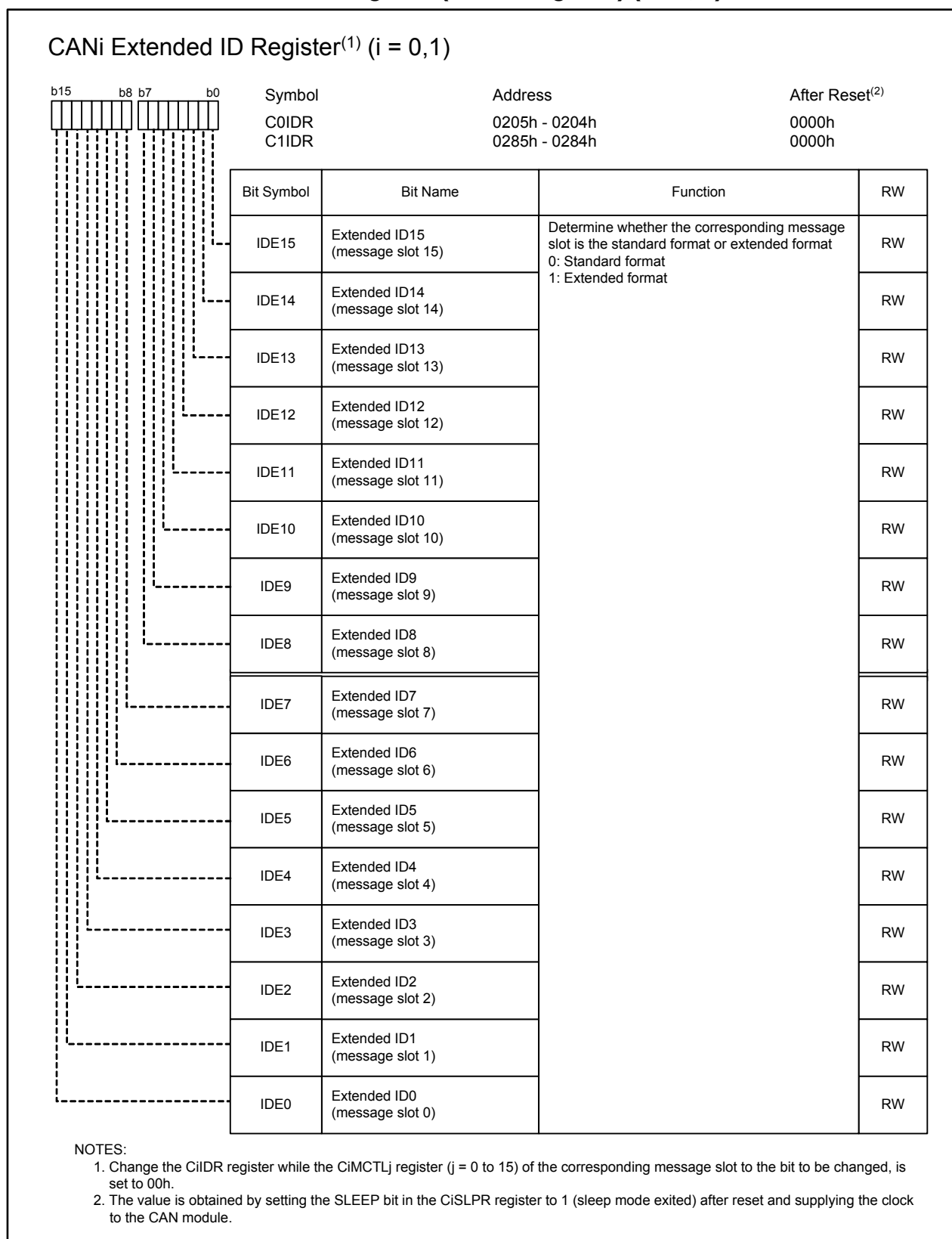
Figure 23.7 C0IDR and C1IDR Registers
