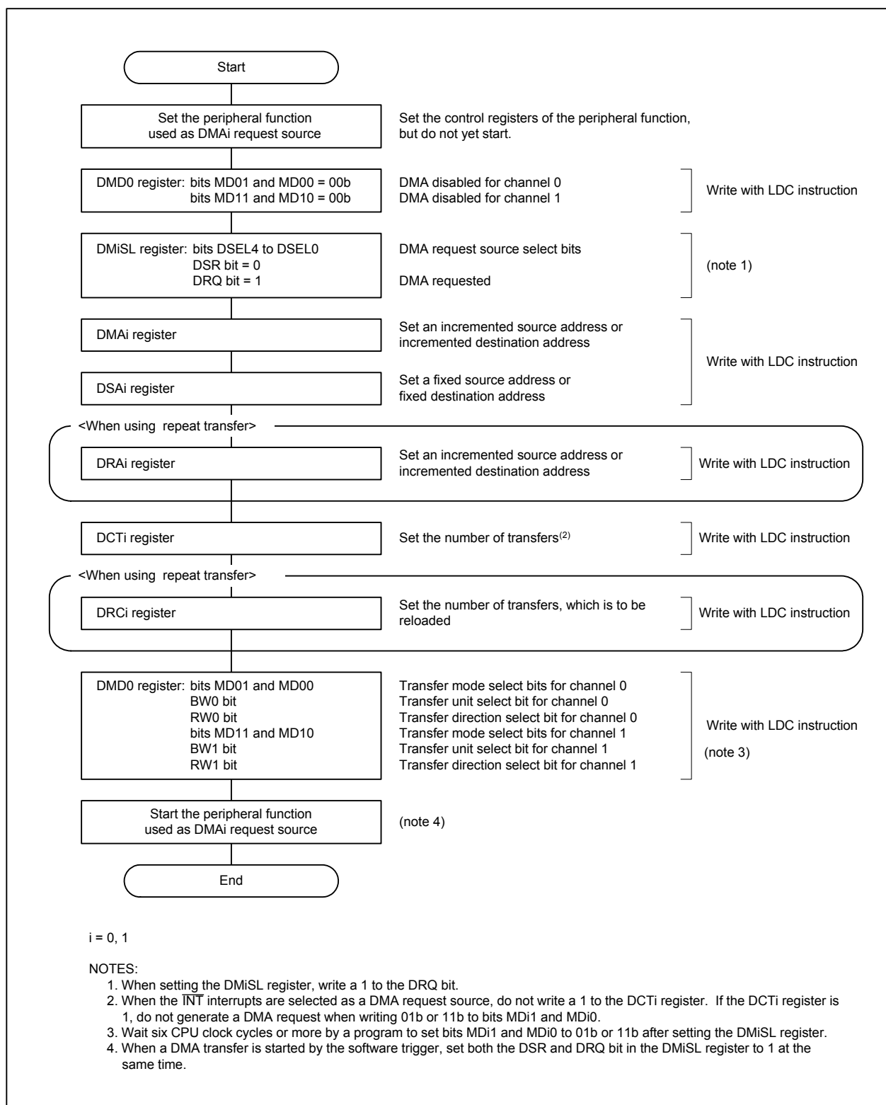
Figure 13.7 Register Settings When Using DMA0 or DMA1
