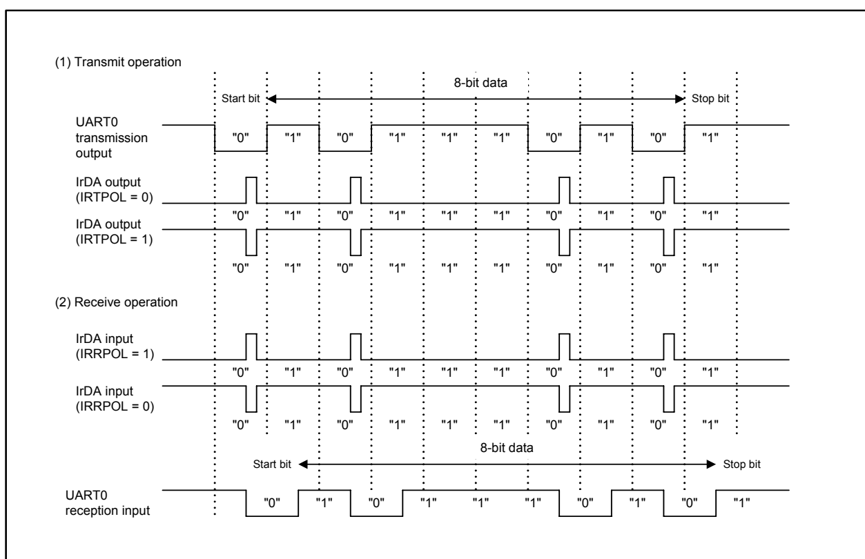
Figure 17.39 IrDA Operation
