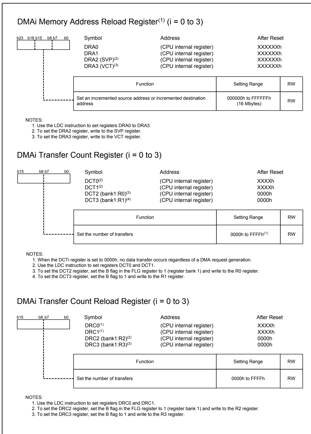
Figure 13.4 DRA0 to DRA3 Registers, DCT0 to DCT3 Registers, DRC0 to DRC3 Registers
