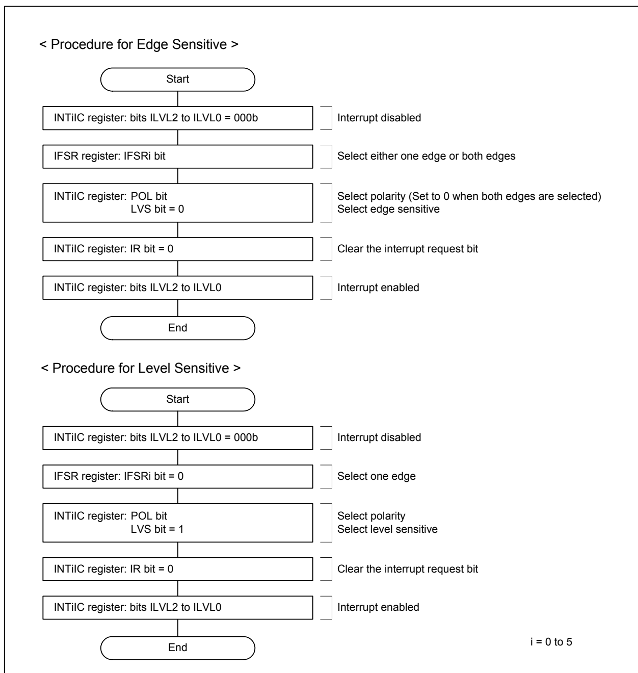
Figure 28.3 Procedure to set the INT i Interrupt Source (i = 0 to 5)
