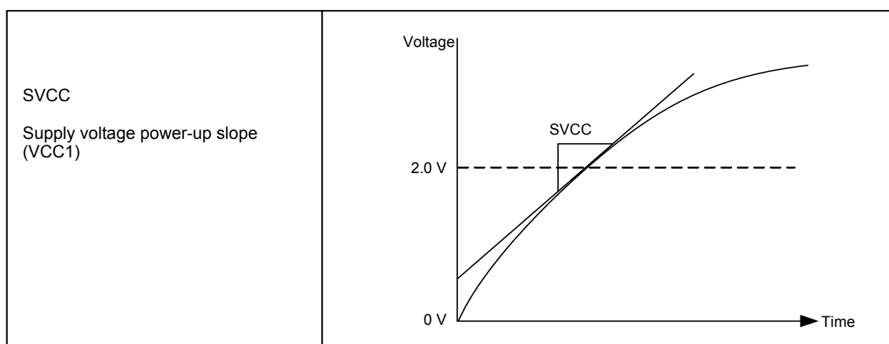
Figure 28.1 SVCC Timing
