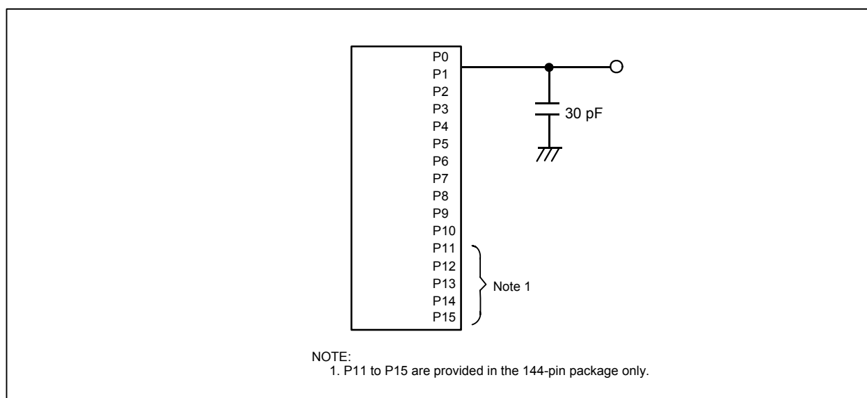
Figure 27.2 P0 to P15 Measurement Circuit
