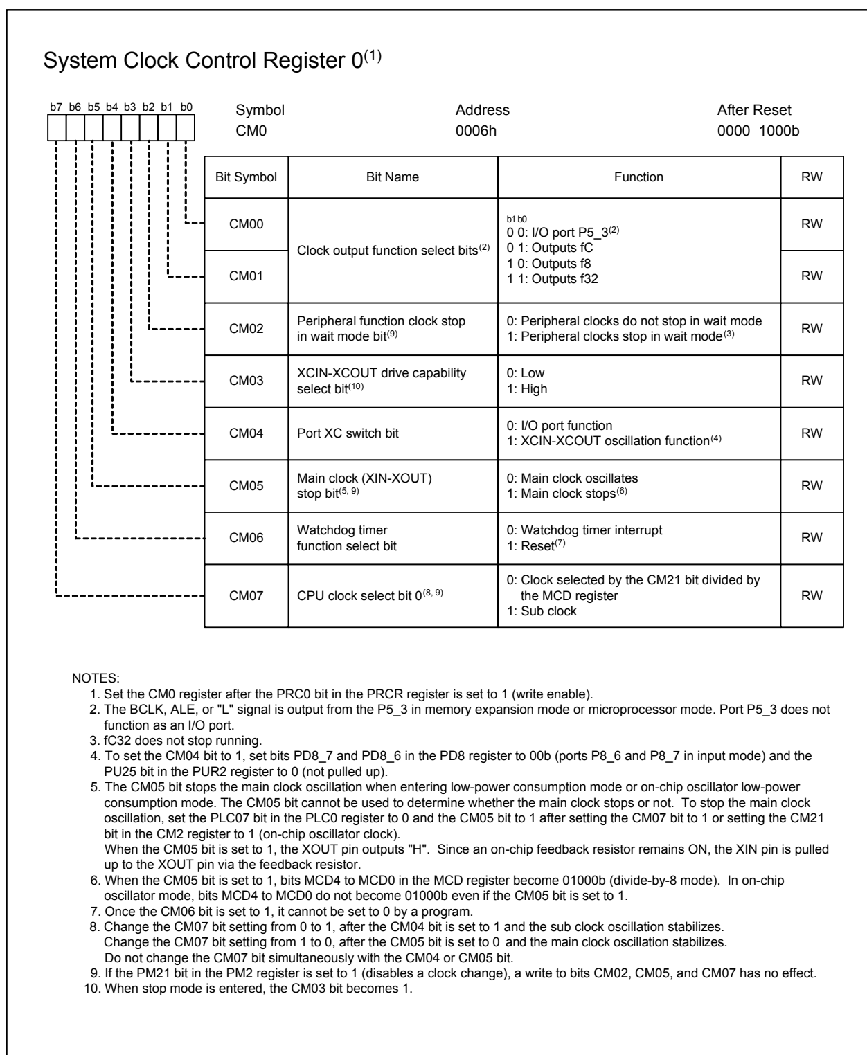
Figure 9.2 CM0 Register
