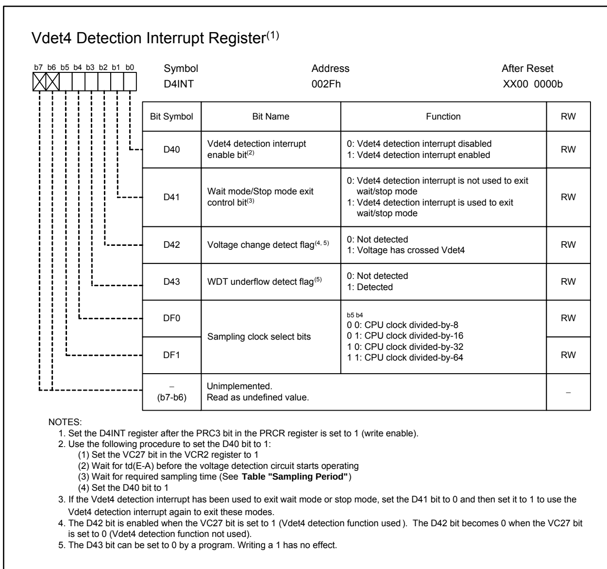
Figure 6.3 D4INT Register
