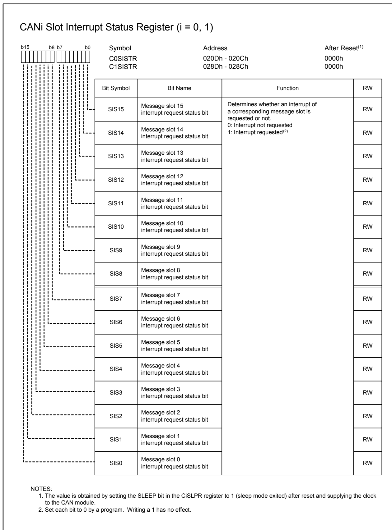
Figure 23.14 C0SISTR and C1SISTR Registers
