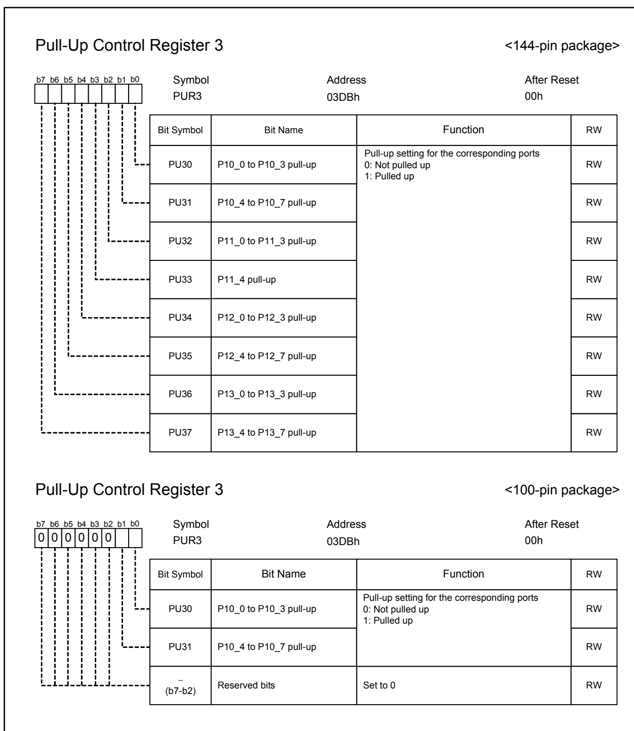
Figure 25.22 PUR3 Register
