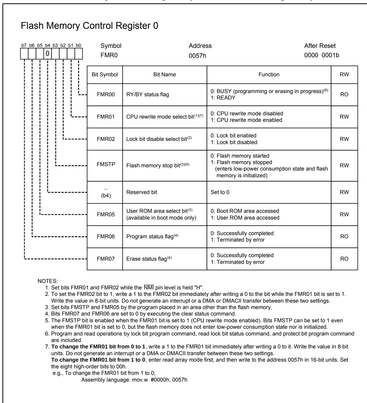
Figure 26.4 FMR0 Register
