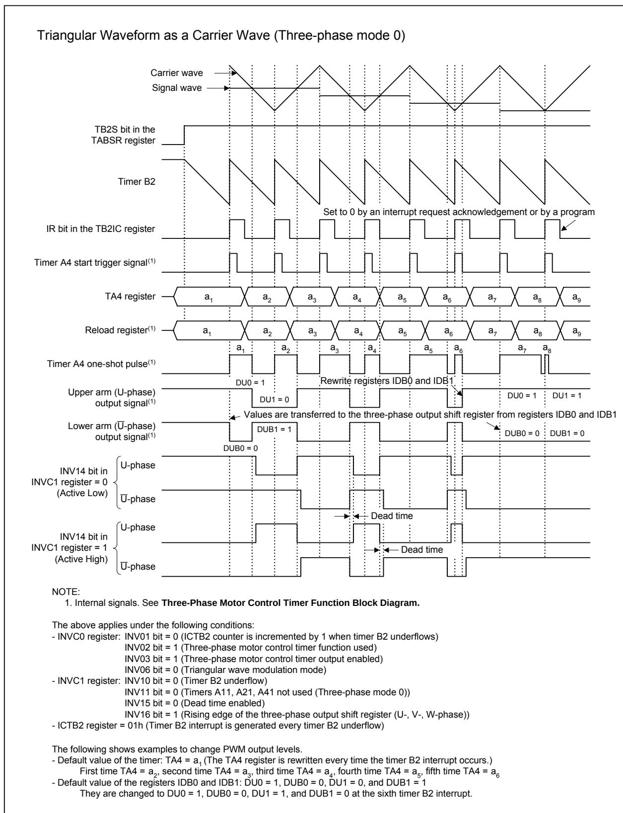
Figure 16.11 Triangular Wave Modulation Operation (Three-Phase Mode 0)
