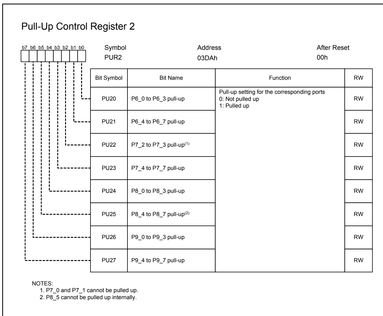
Figure 25.21 PUR2 Register
