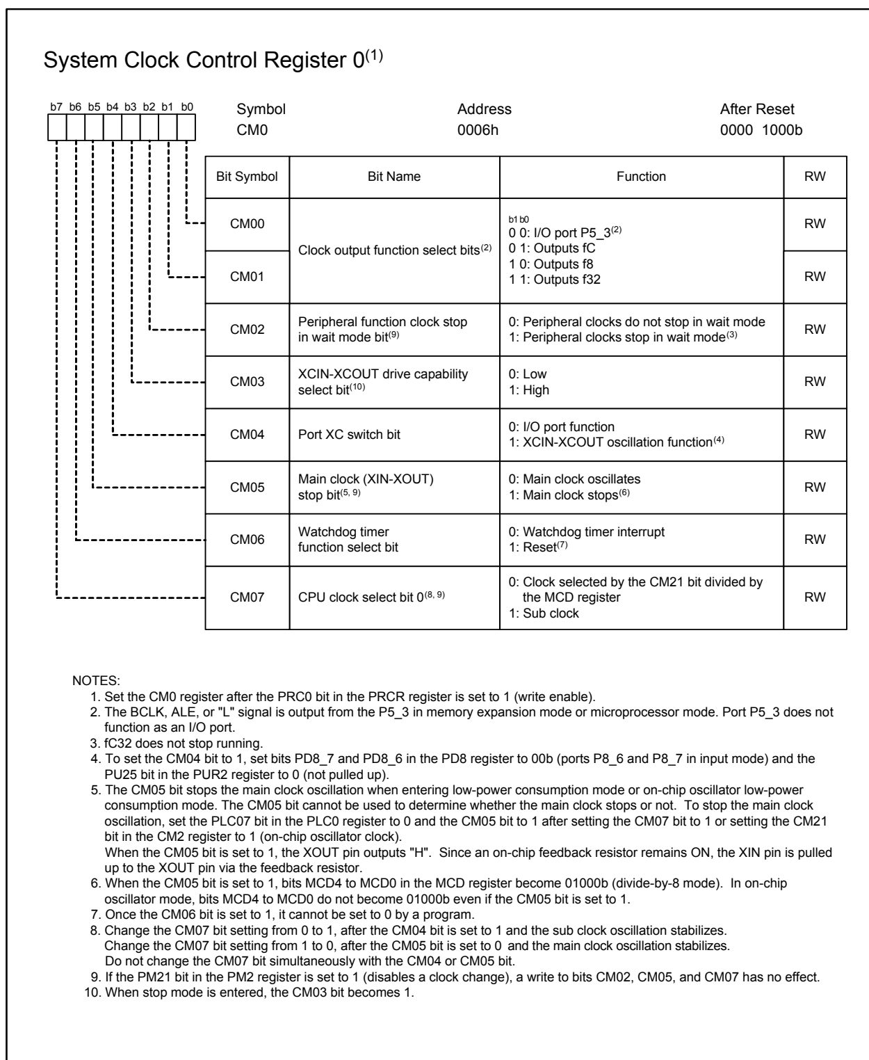
Figure 12.2 CM0 Register
