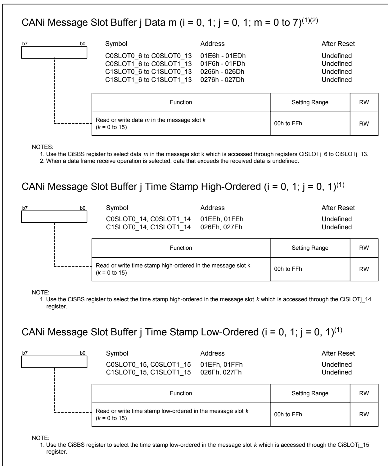
Figure 23.35 C0SLOT0_6 to C0SLOT0_13, C0SLOT1_6 to C0SLOT1_13, C1SLOT0_6 to C1SLOT0_13, and C1SLOT1_6 to C1SLOT1_13 Registers, C0SLOT0_14, C0SLOT1_14, C1SLOT0_14, and C1SLOT1_14 Registers C0SLOT0_15, C0SLOT1_15, C1SLOT0_15, and C1SLOT1_15 Registers
