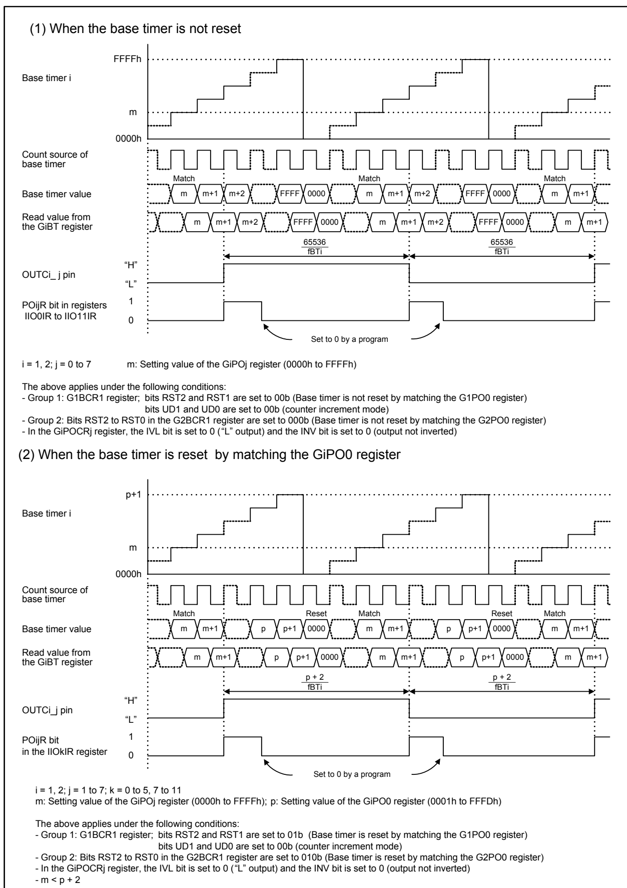
Figure 22.28 Phase-Delayed Waveform Output Mode Operation
