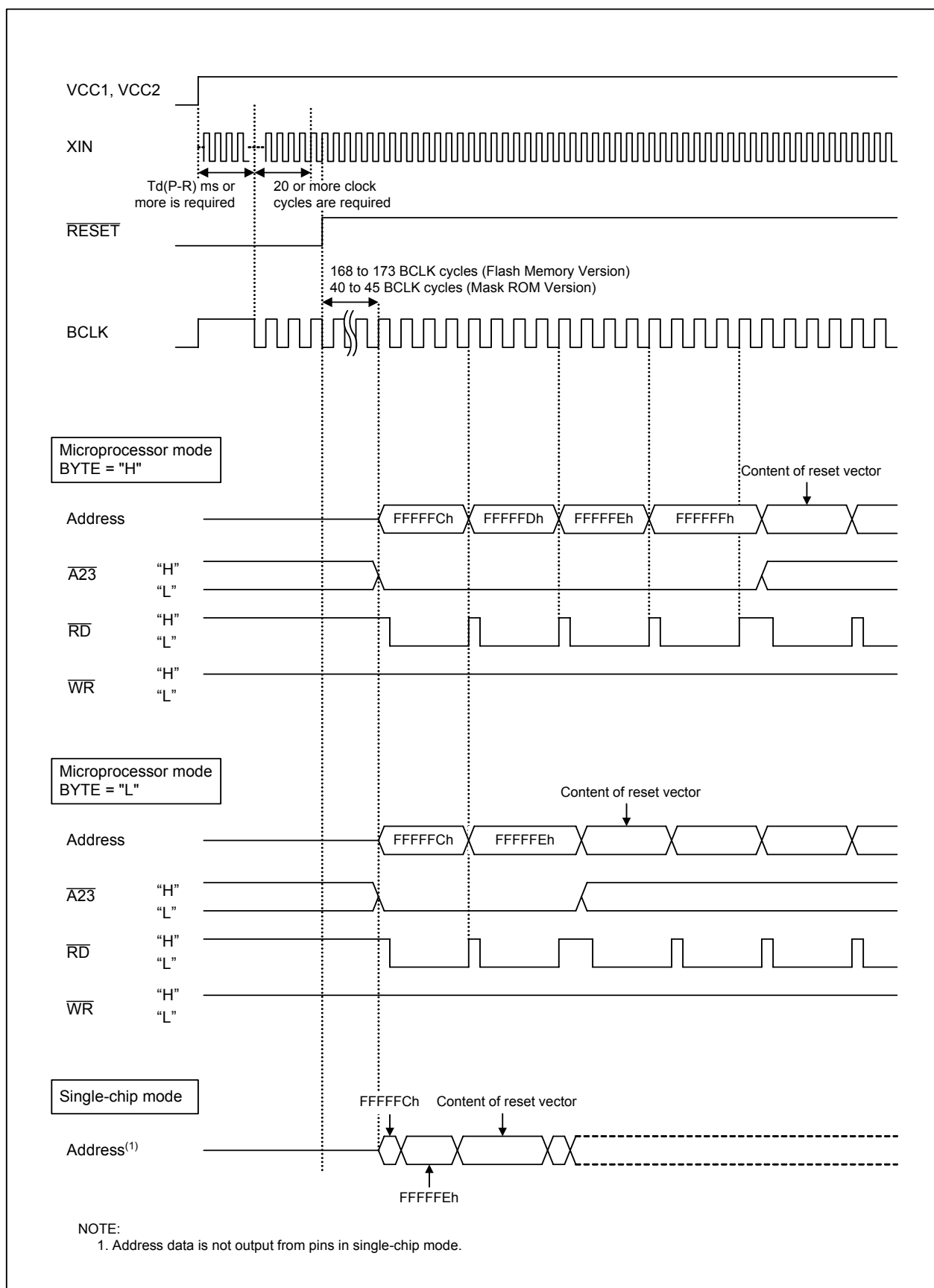
Figure 5.2 Reset Sequence
