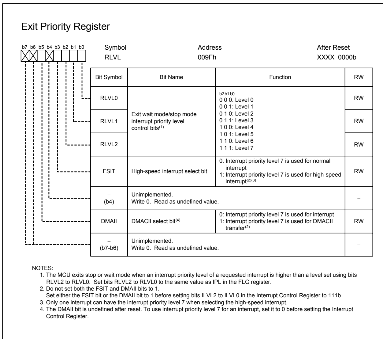
Figure 11.6 RLVL Register
