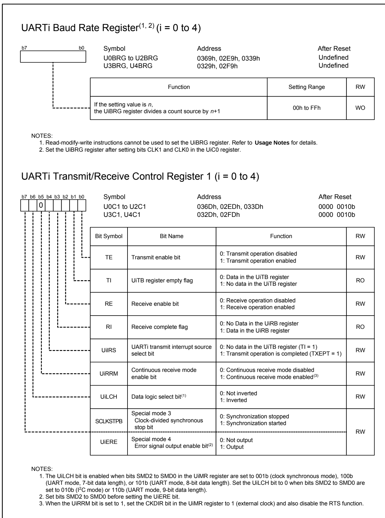
Figure 17.8 U0BRG to U4BRG Registers, U0C1 to U4C1 Registers
