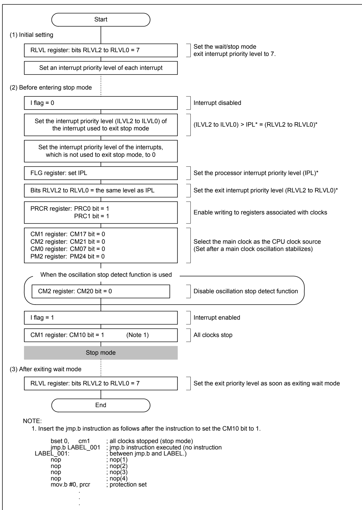
Figure 9.15 Procedure to Enter Stop Mode
