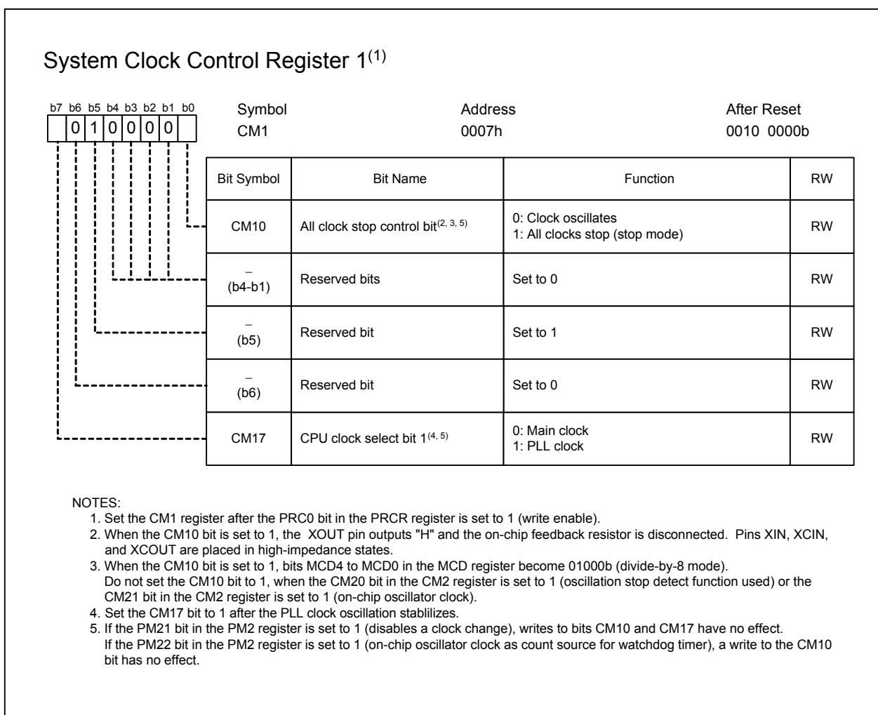
Figure 9.3 CM1 Register
