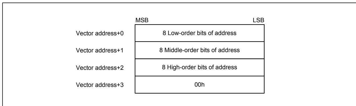
Figure 11.3 Interrupt Vector
