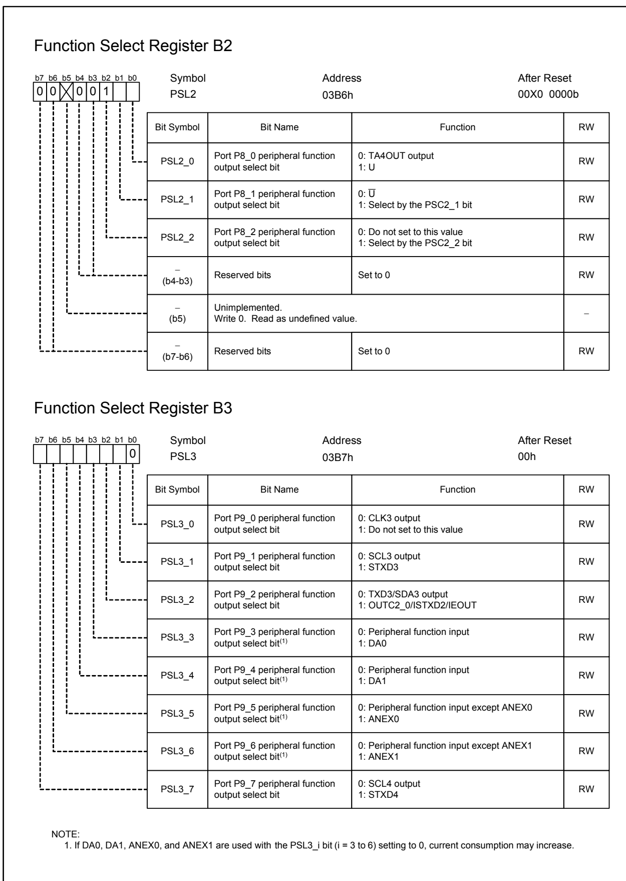
Figure 25.13 PSL2 Register, PSL3 Register
