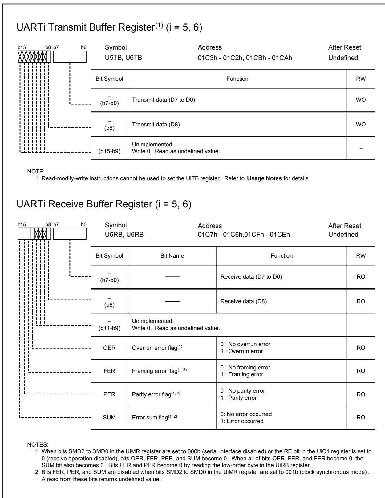
Figure 17.45 U5TB and U6TB Registers, U5RB and U6RB Registers
