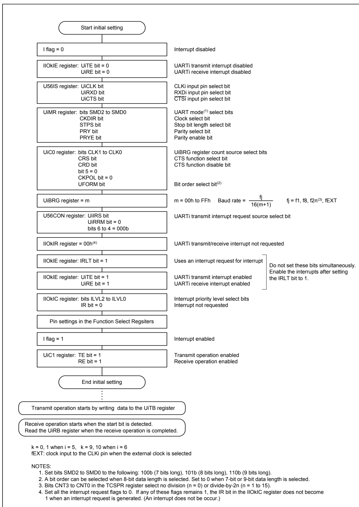
Figure 17.51 Register Settings in UART Mode
