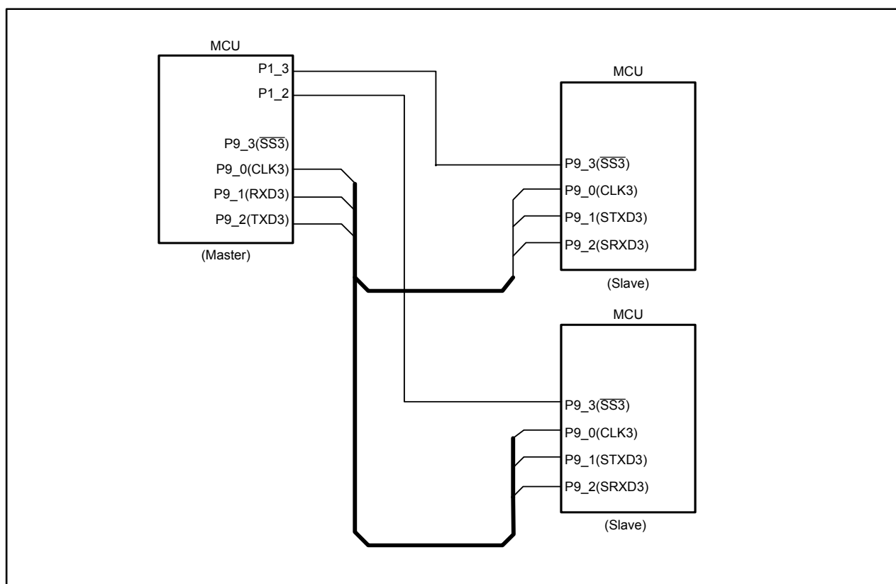
Figure 17.28 Serial Bus Communication Control with \overline{\text{SSi}} Pin
