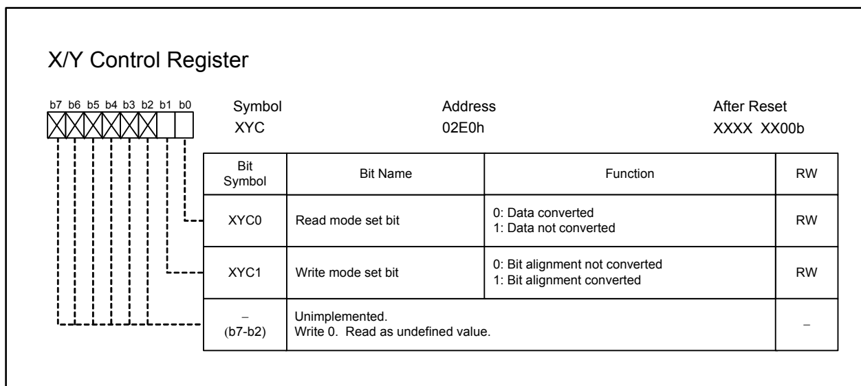
Figure 21.1 XYC Register
