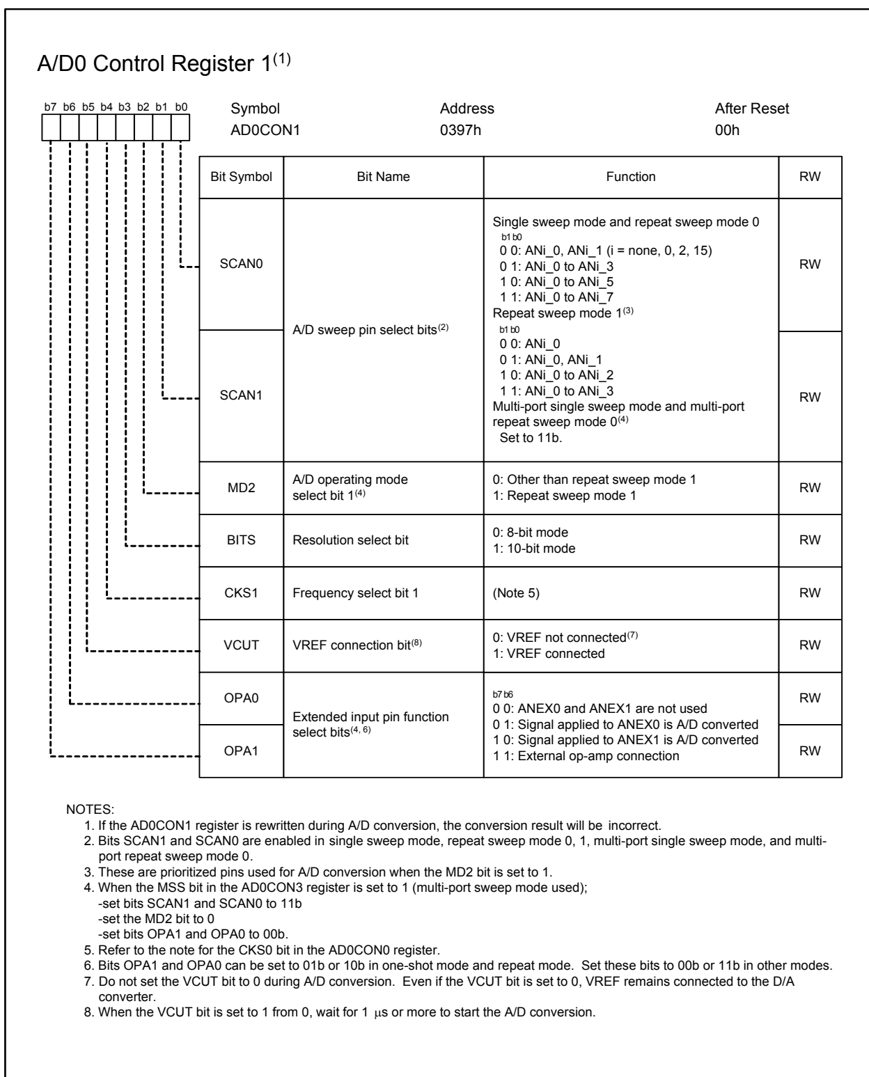
Figure 18.3 AD0CON1 Register
