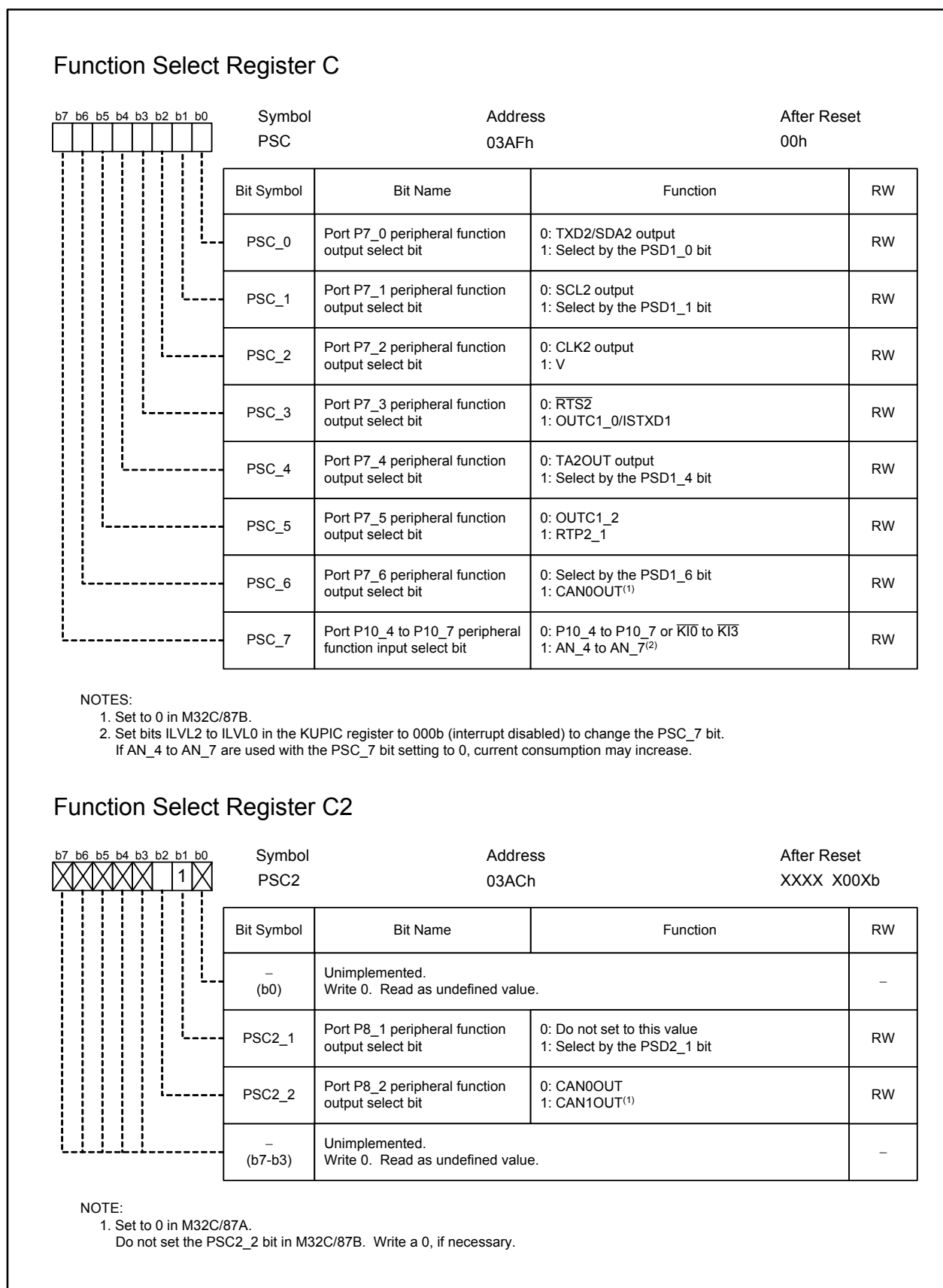
Figure 25.16 PSC Register, PSC2 Register
