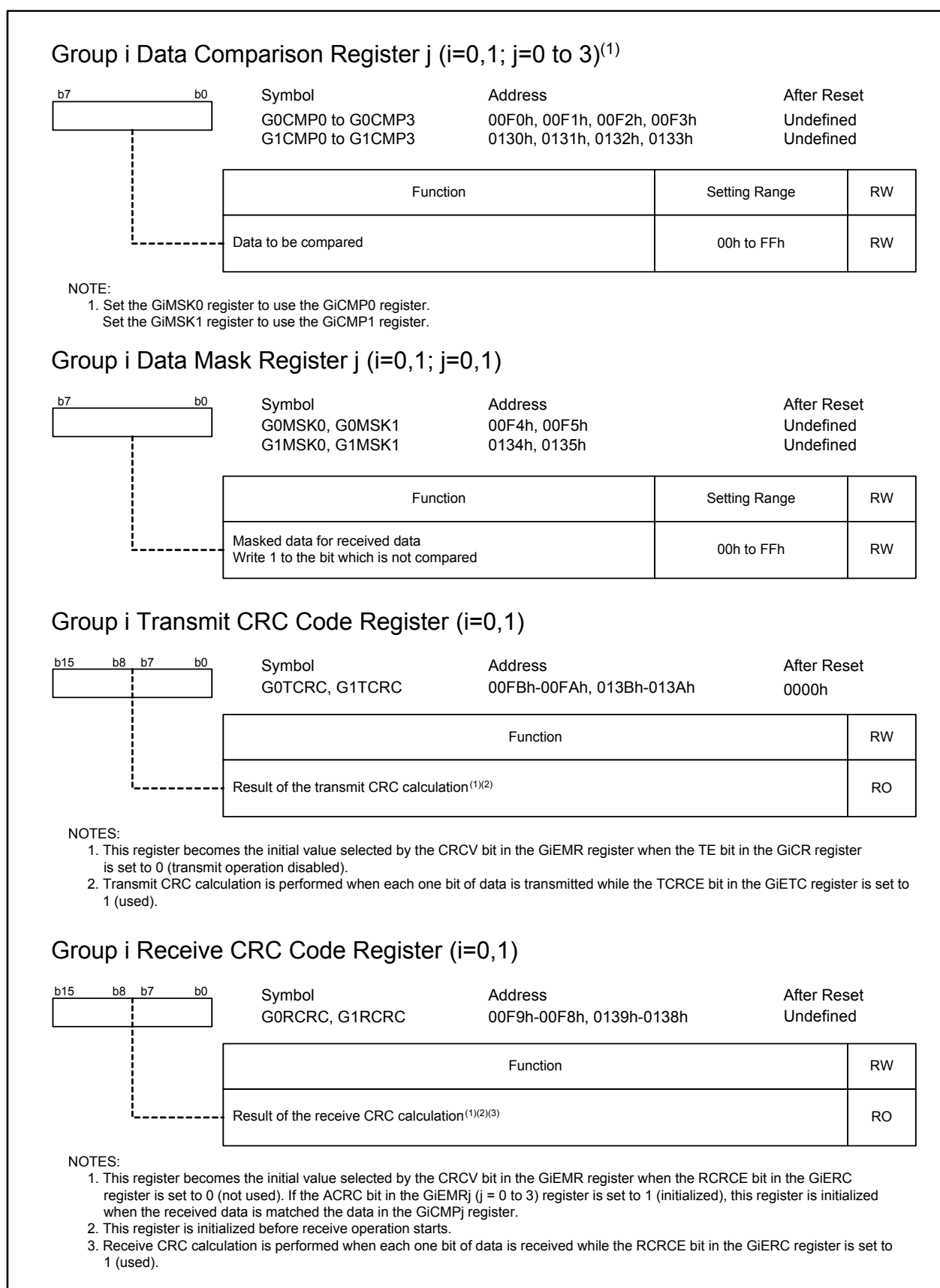
Figure 22.44 G0CMP0 to G0CMP3, G1CMP0 to G1CMP3 Registers, G0MSK0 and G0MSK1 Registers, G1MSK0 and G1MSK1 Registers, G0TCRC and G1TCRC Registers, G0RCRC and G1RCRC Registers
