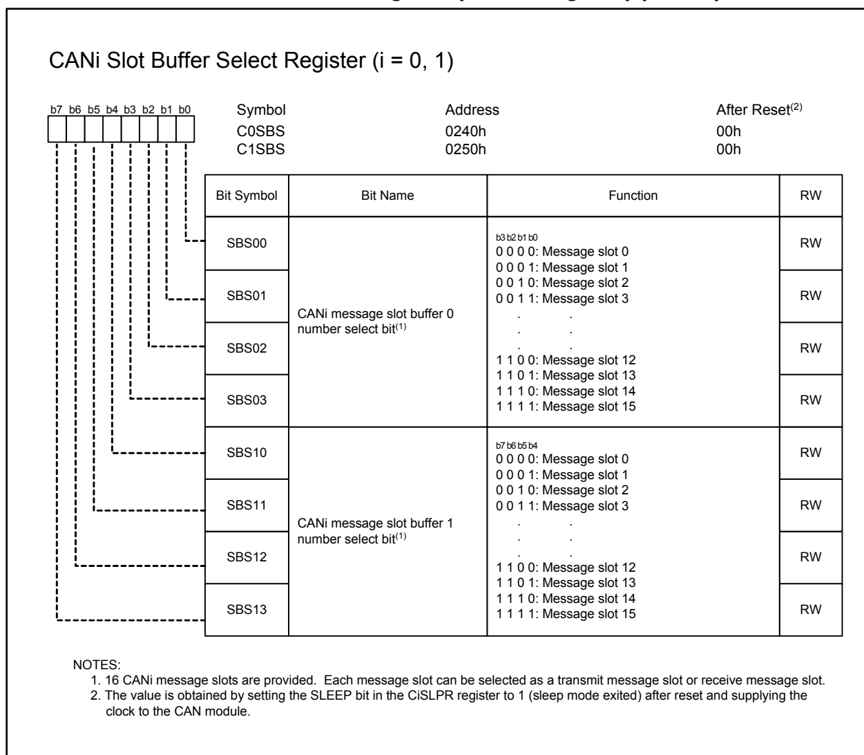
Figure 23.31 C0SBS and C1SBS Registers
