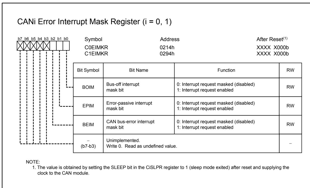
Figure 23.16 C0EIMKR and C1EIMKR Registers
