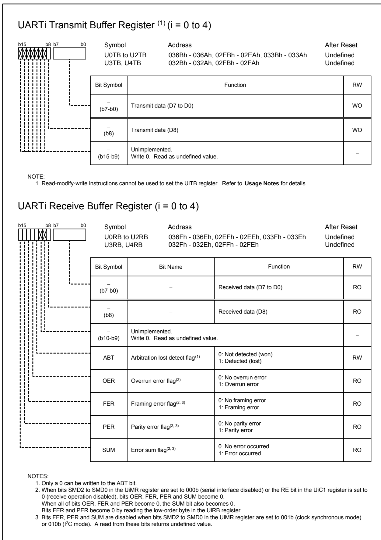
Figure 17.10 U0TB to U4TB Registers, U0RB to U4RB Registers
