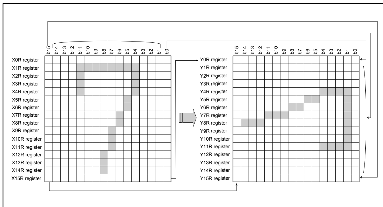
Figure 21.3 X/Y Conversion
