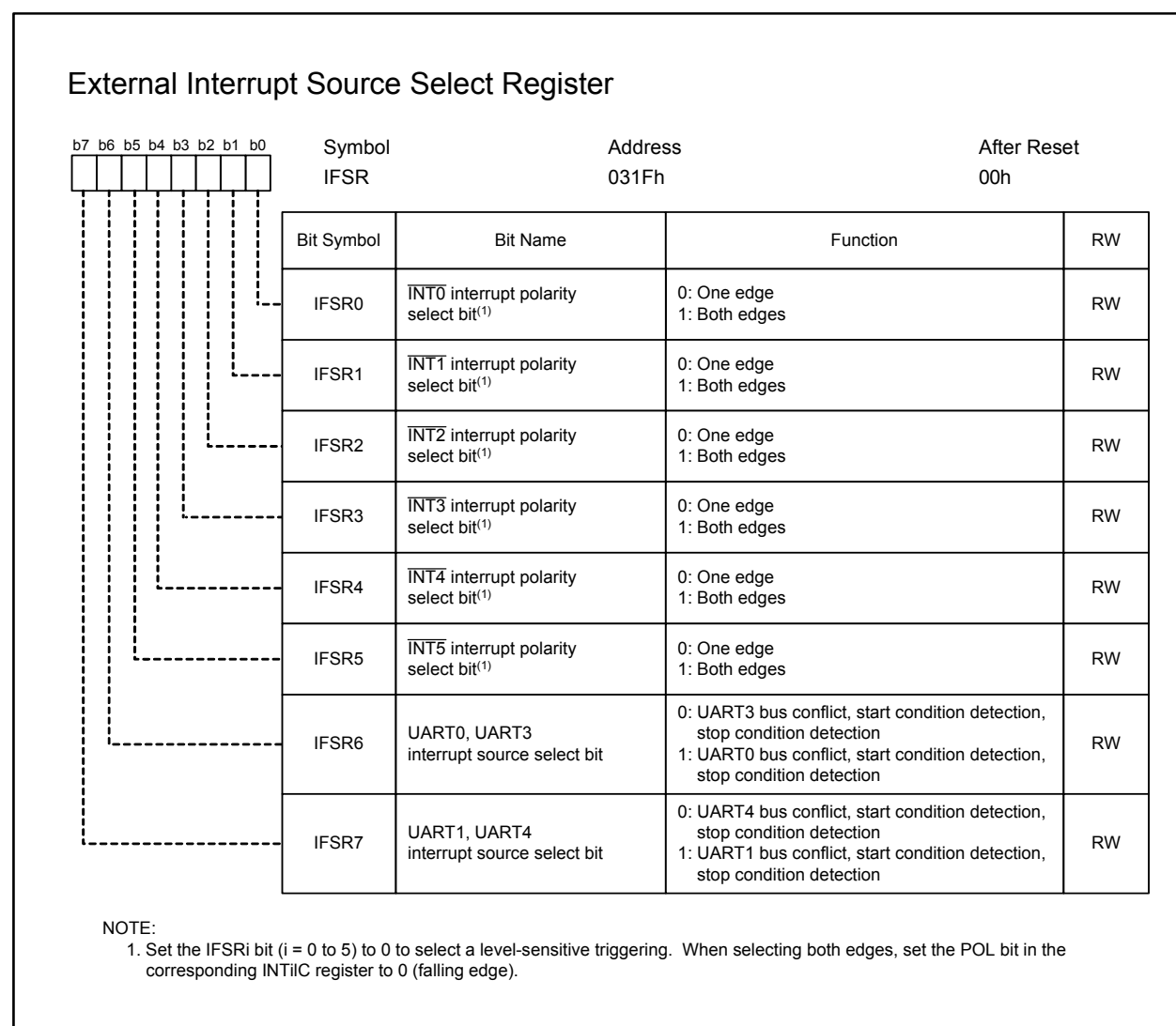
Figure 11.13 IFSR Register
