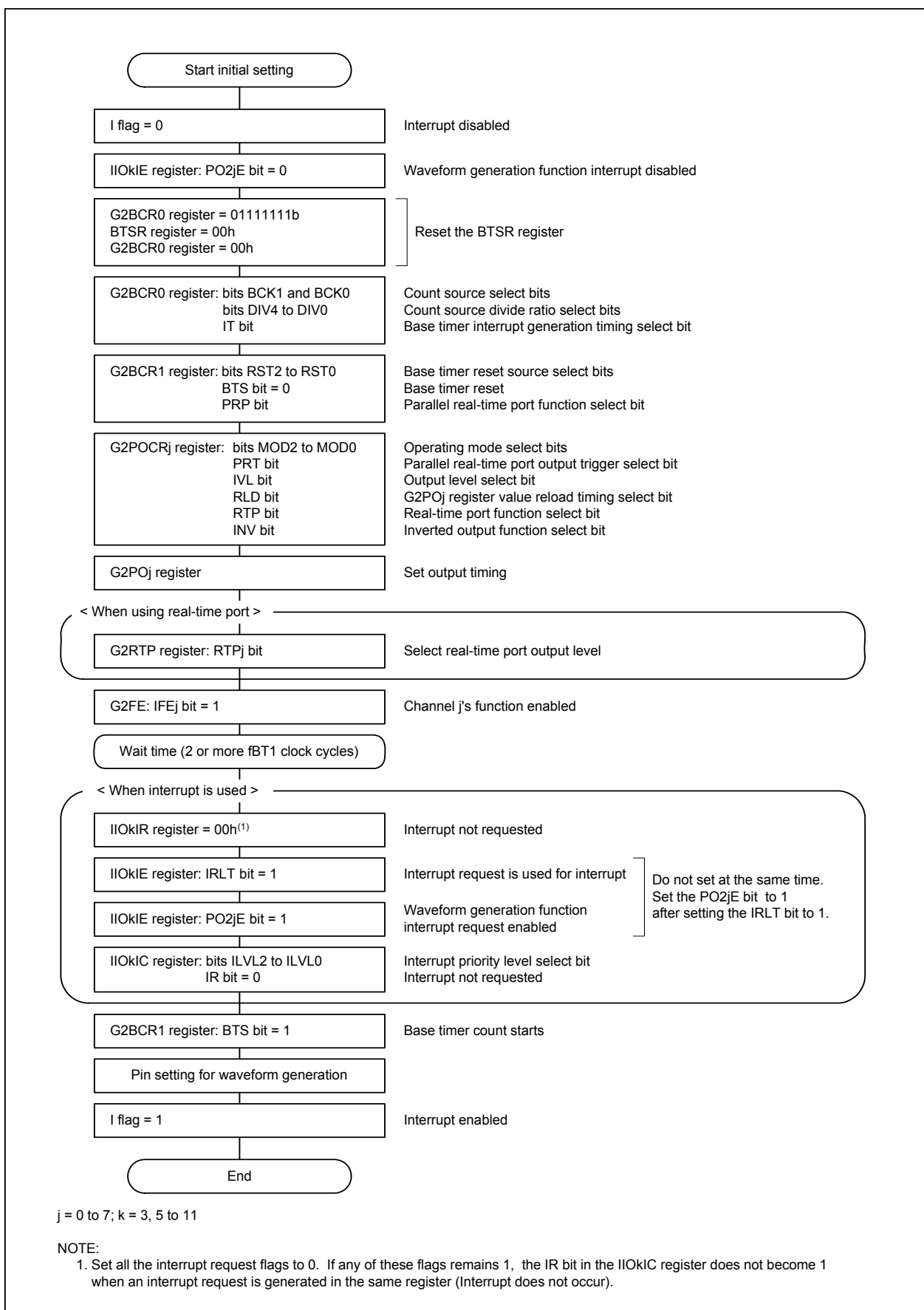
Figure 22.26 Register Settings for Waveform Generation Function (Group 2)
