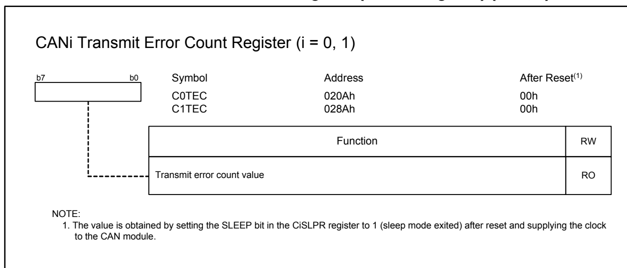
Figure 23.12 C0TEC and C1TEC Registers
