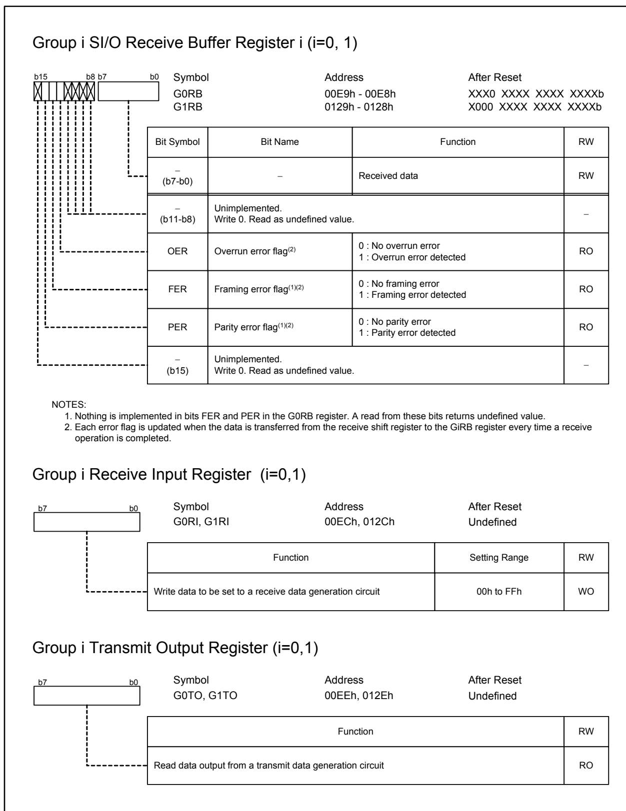
Figure 22.46 G0RB, G1RB Registers, G0RI, G1RI Registers, G0TO, G1TO Registers
