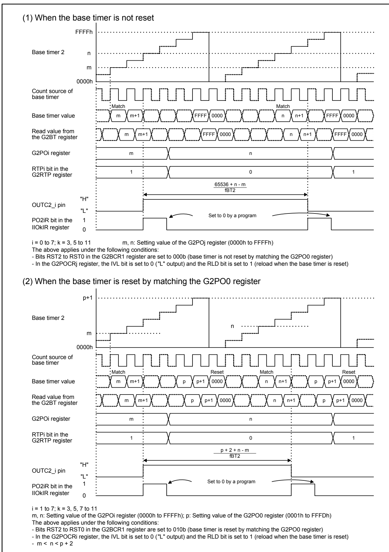
Figure 22.32 Real-Time Port Output Mode Operation
