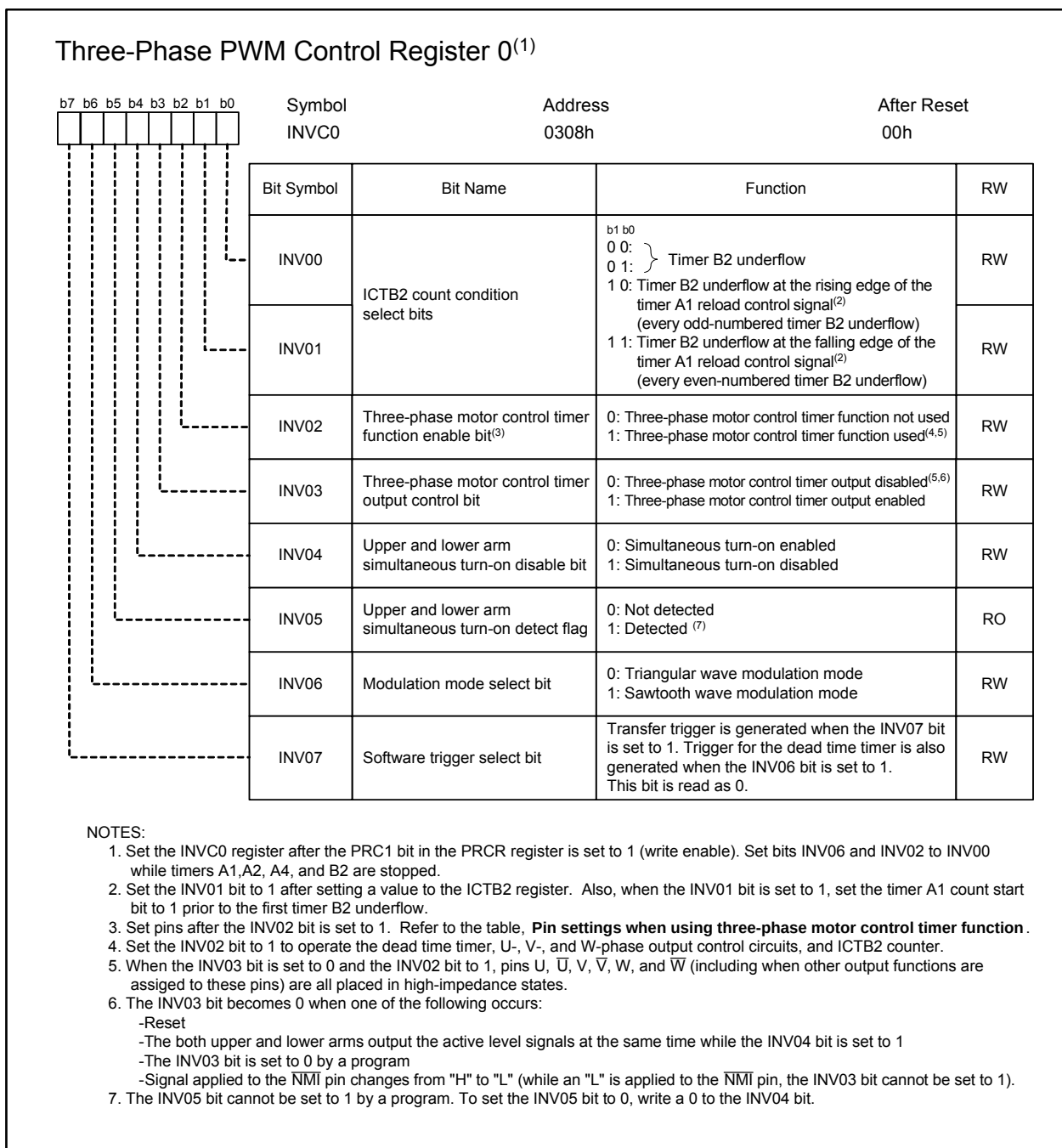
Figure 16.2 INVC0 Register
