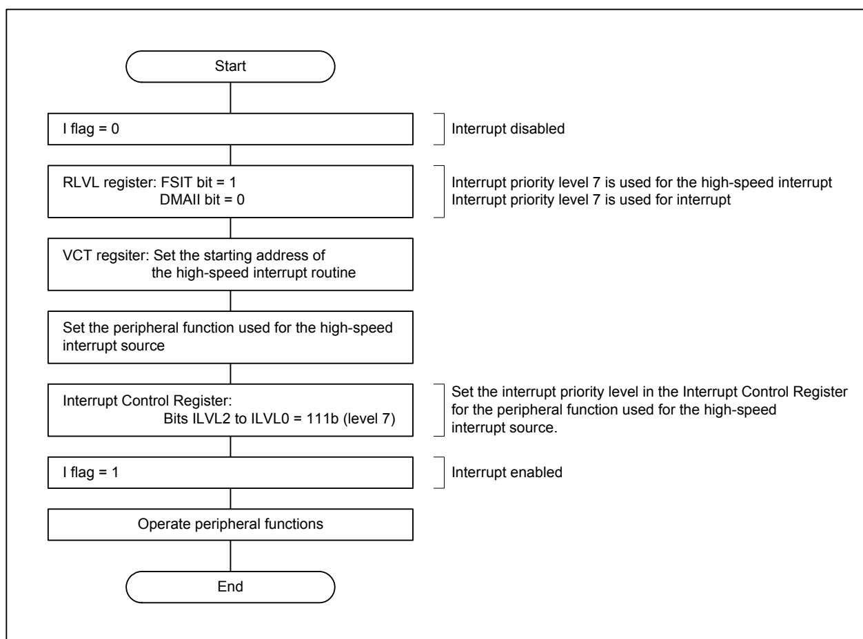
Figure 11.2 Procedure to Use High-Speed Interrupt
