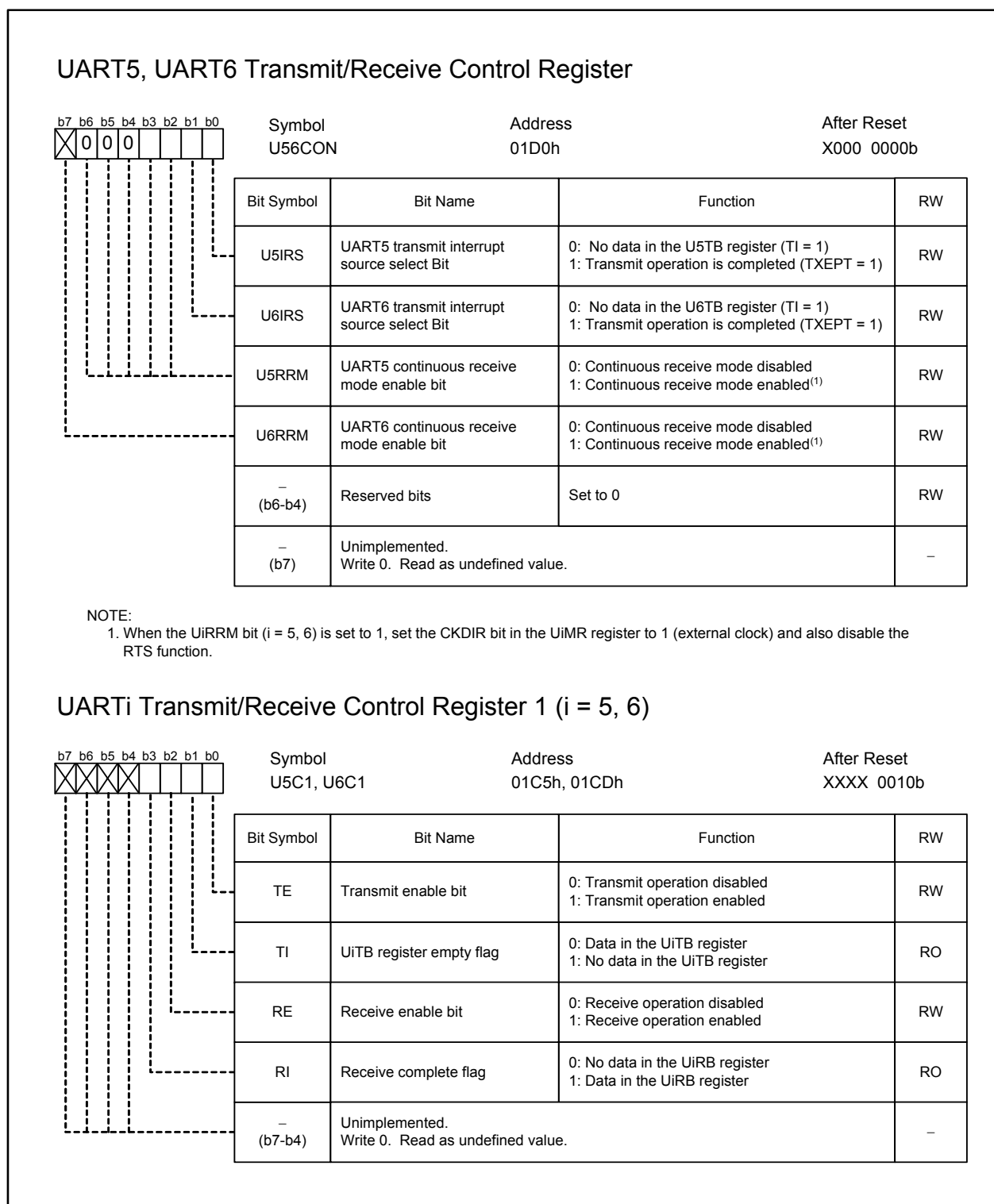
Figure 17.44 U56CON Register, U5C1 and U6C1 Registers
