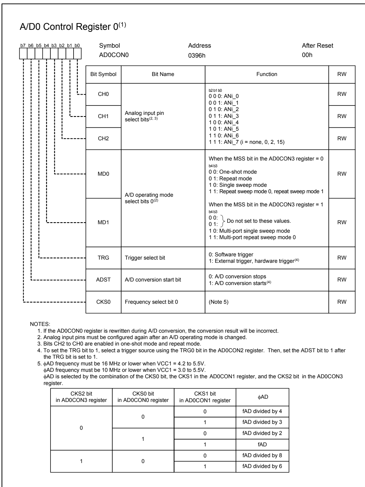
Figure 18.2 AD0CON0 Register
