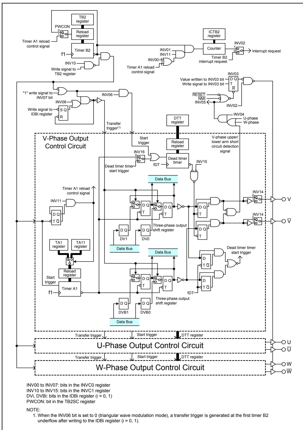
Figure 16.1 Three-Phase Motor Control Timer Function Block Diagram
