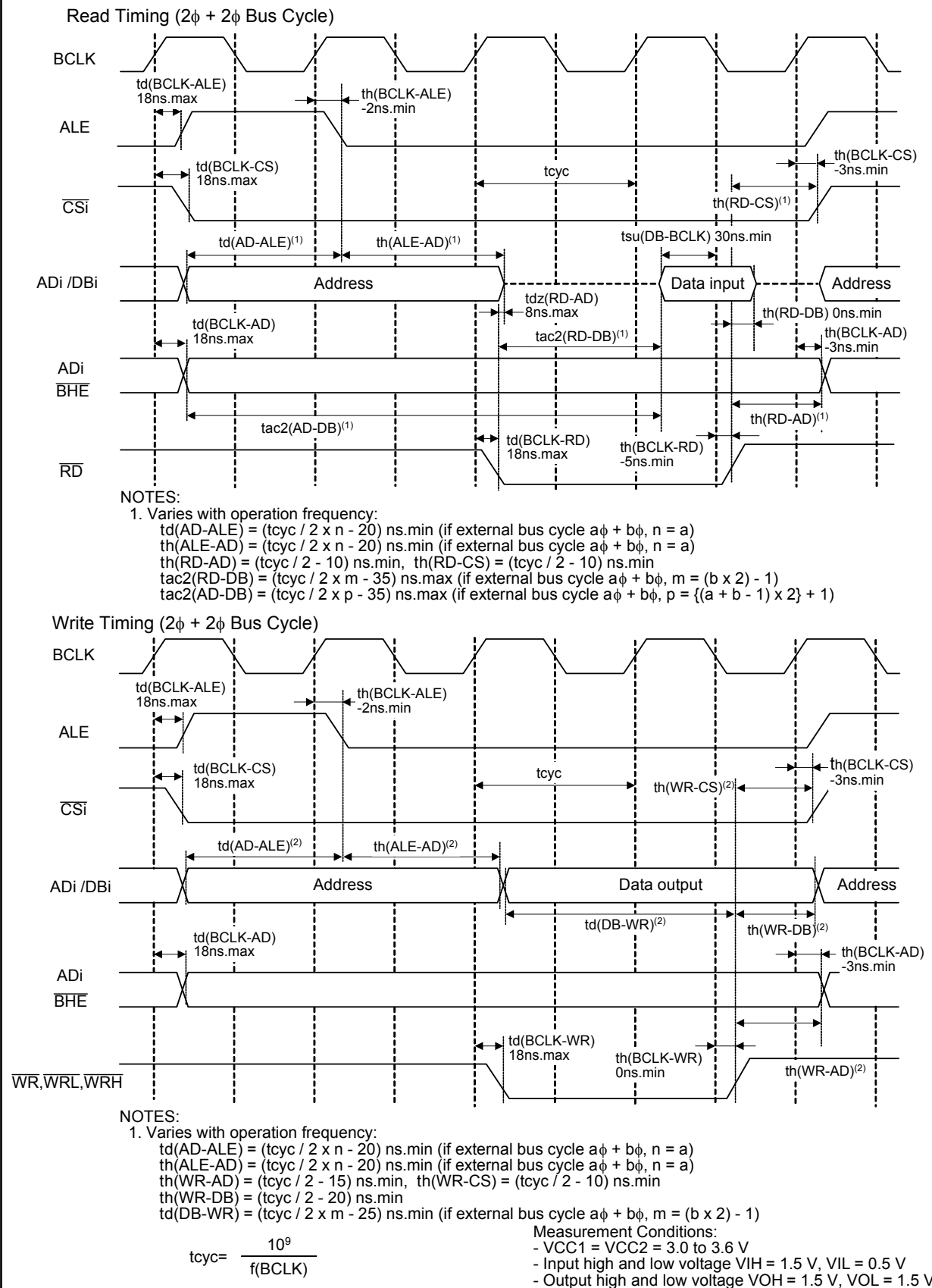
Figure 27.10 VCC1 = VCC2 = 3.3 V Timing Diagram (4/4)
