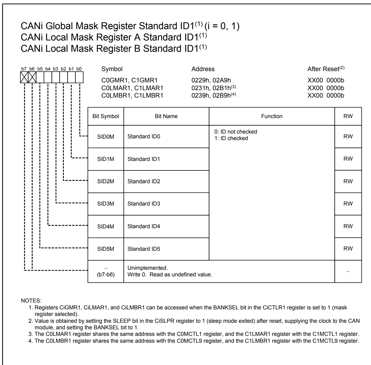
Figure 23.24 C0GMR1, C1GMR1, C0LMAR1, C1LMAR1, C0LMBR1, and C1LMBR1 Registers
