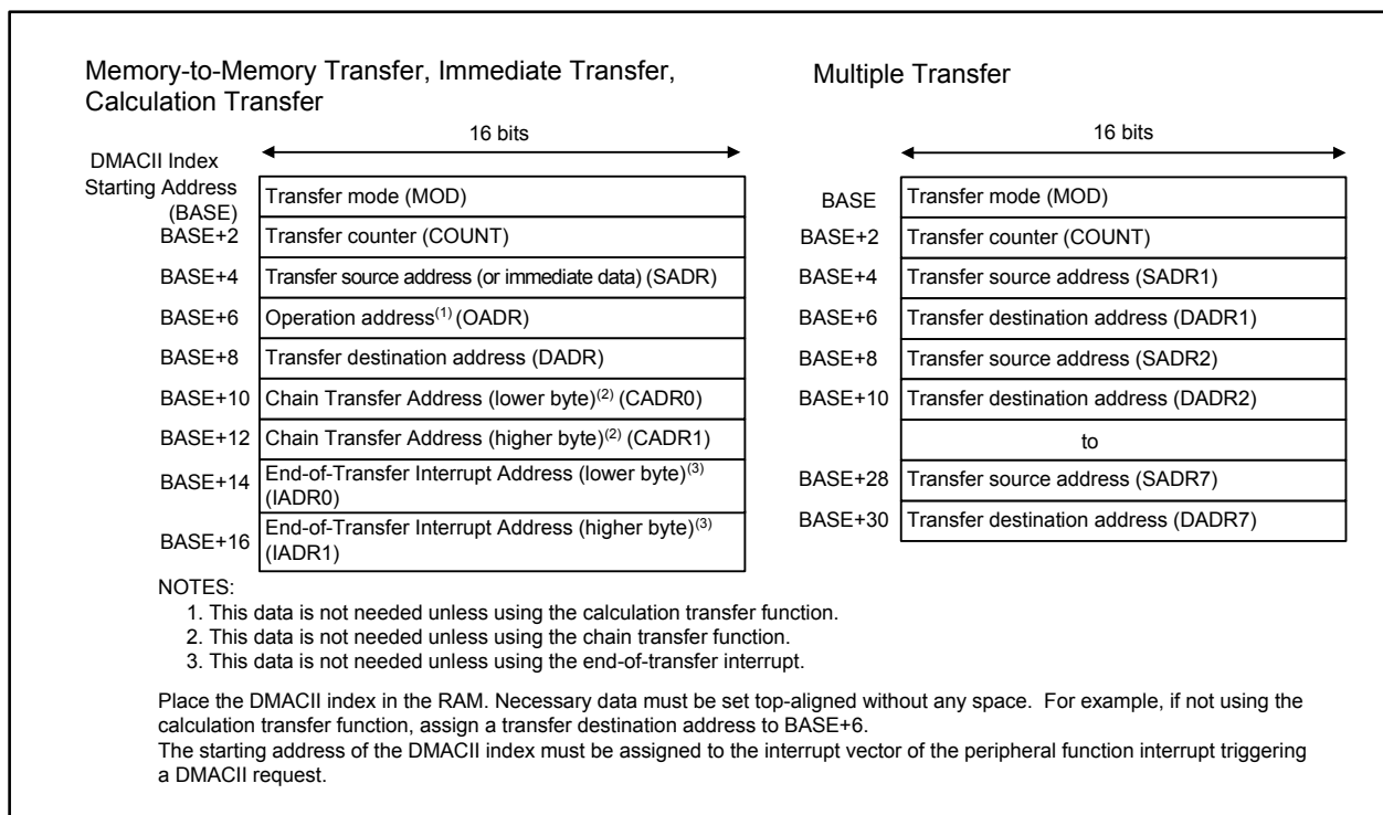
Figure 14.2 DMACII Index
