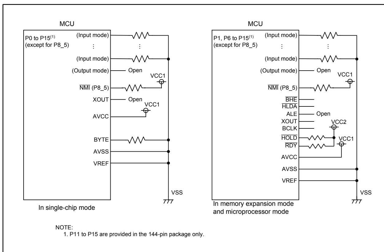
Figure 25.26 Unassigned Pin Handling
