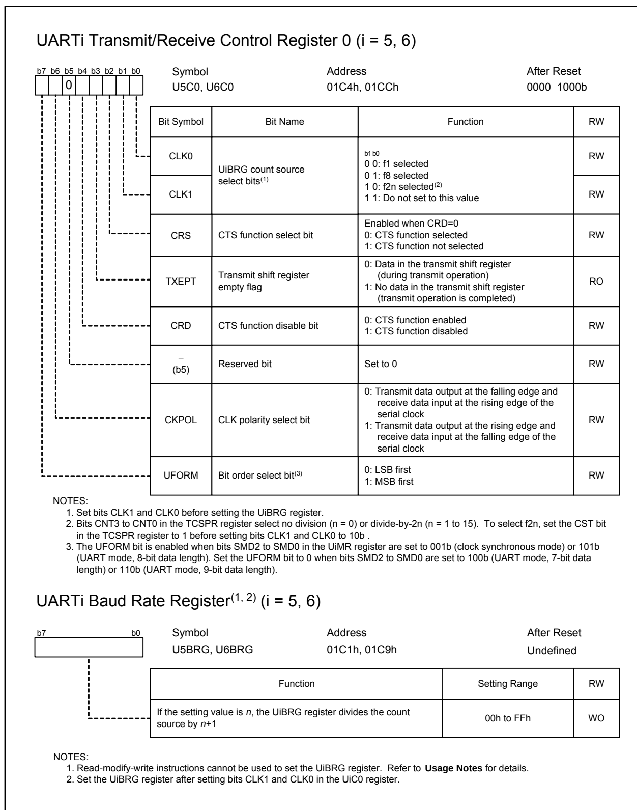
Figure 17.43 U5C0 and U6C0 Registers, U5BRG and U6BRG Registers
