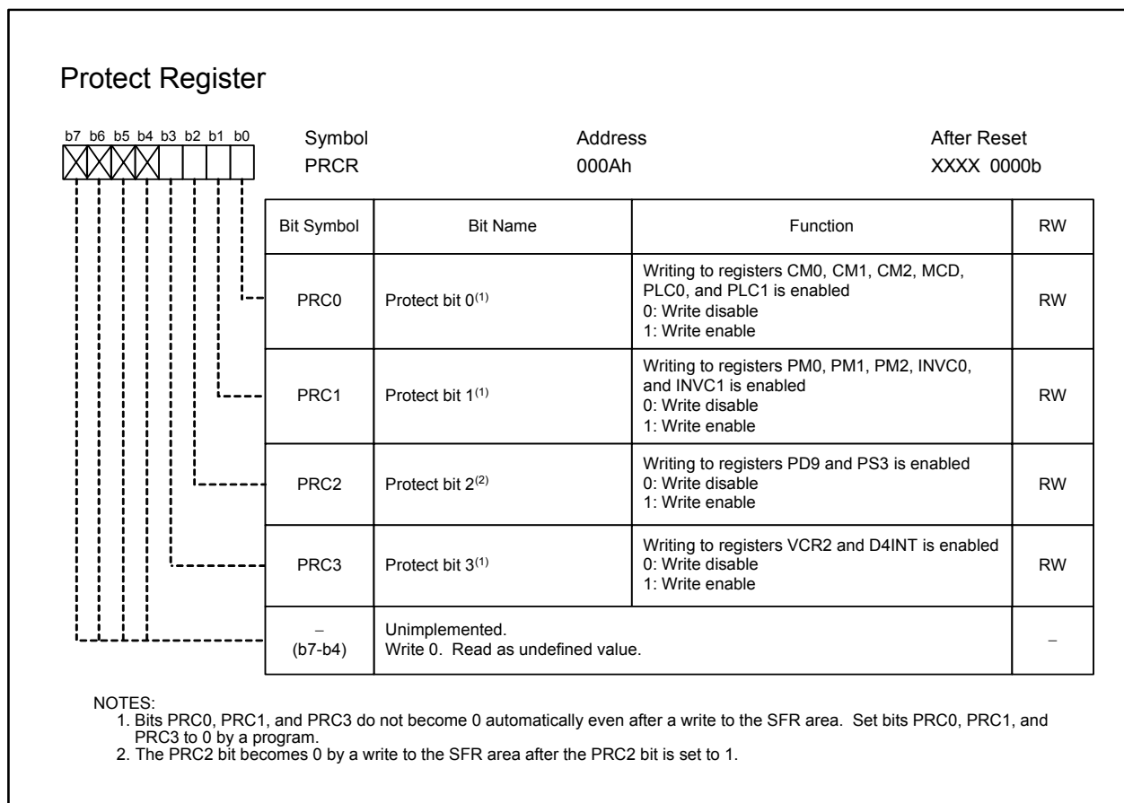
Figure 10.1 PRCR Register
