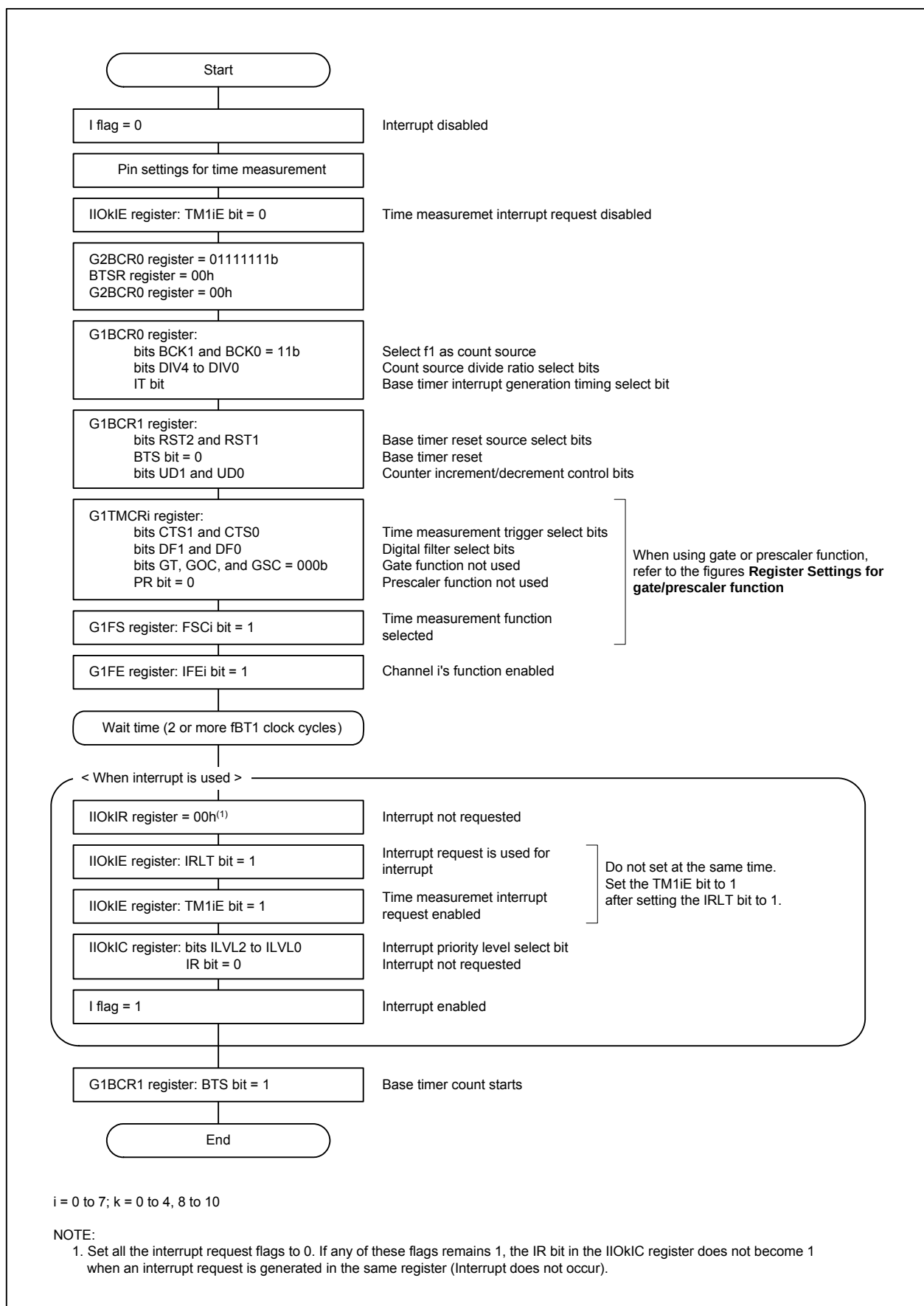
Figure 22.19 Register Settings for Time Measurement Function
