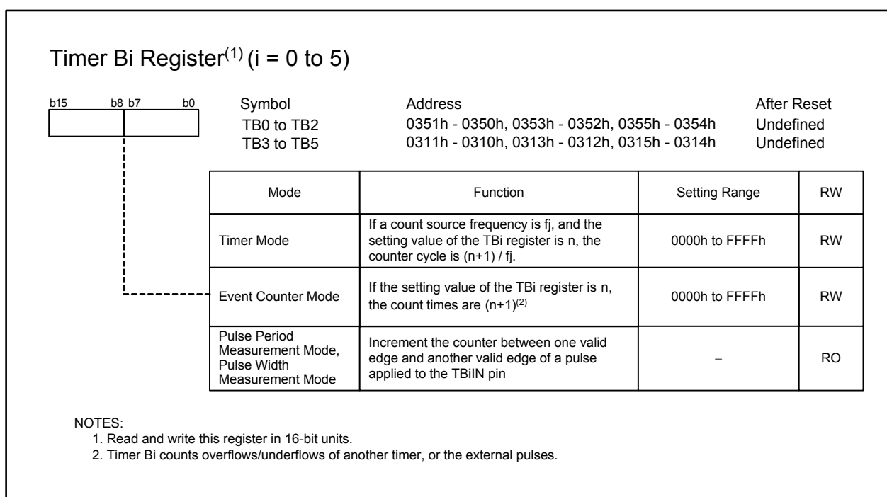
Figure 15.25 TB0 to TB5 Registers
