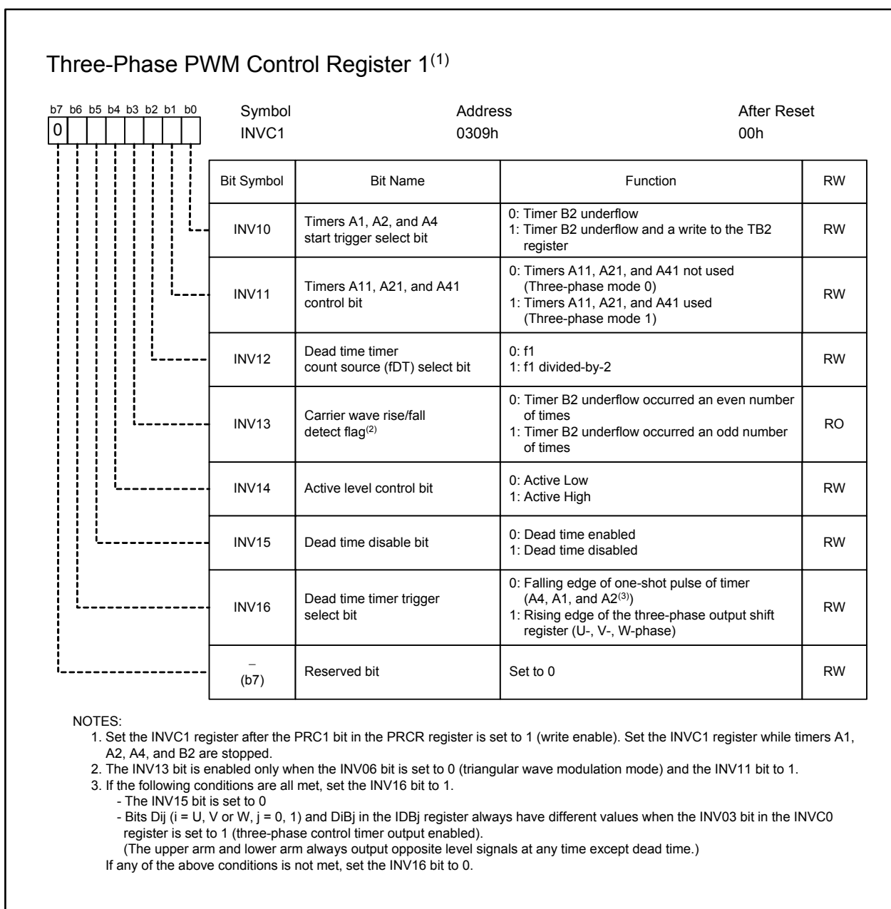
Figure 16.3 INVC1 Register
