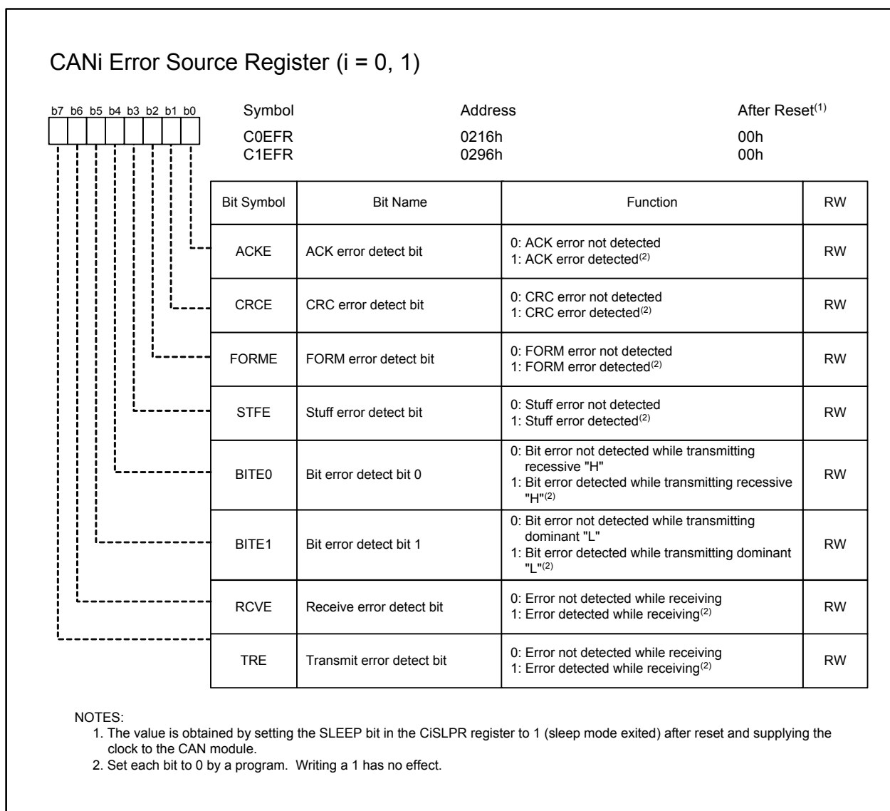
Figure 23.18 C0EFR and C1EFR Registers
