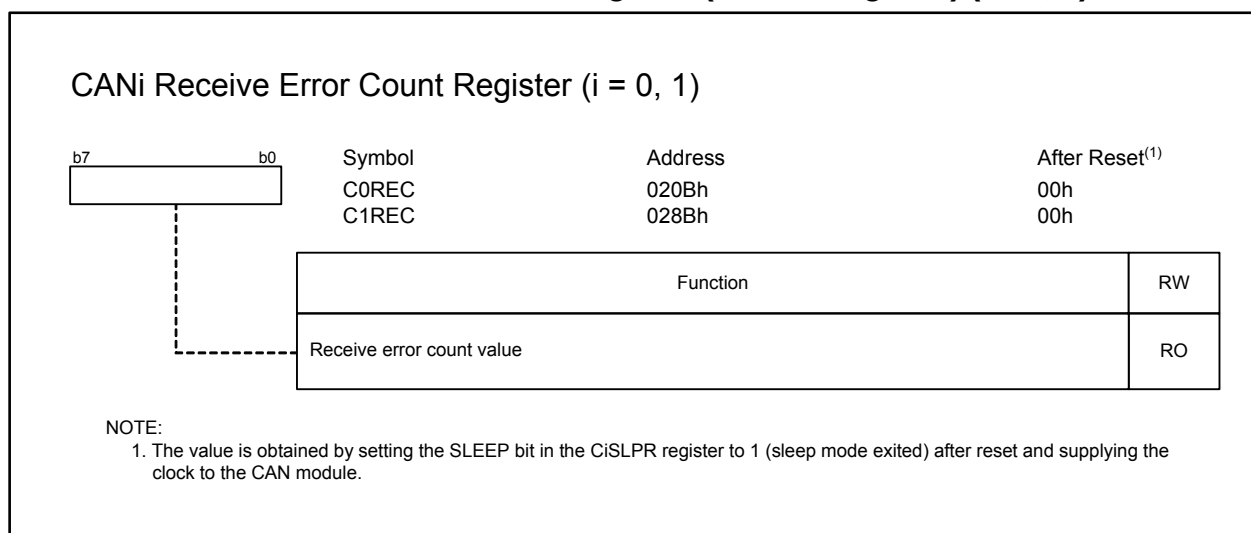
Figure 23.13 C0REC and C1REC Registers
