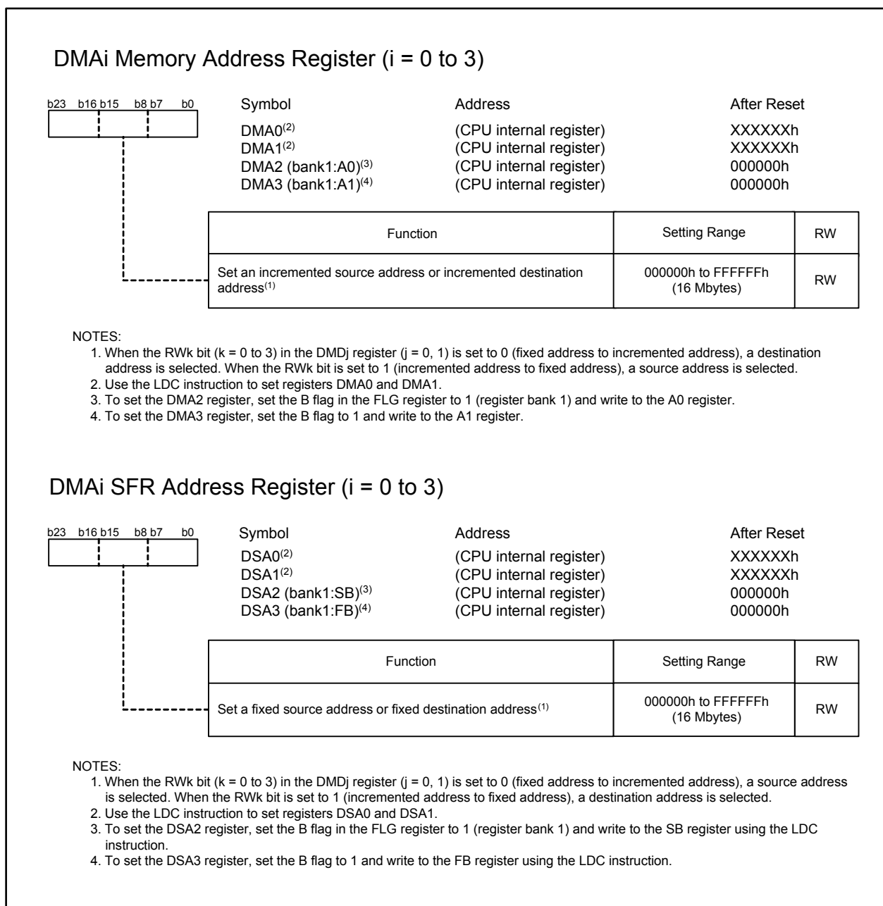
Figure 13.3 DMA0 to DMA3 Registers, DSA0 to DSA3 Registers
