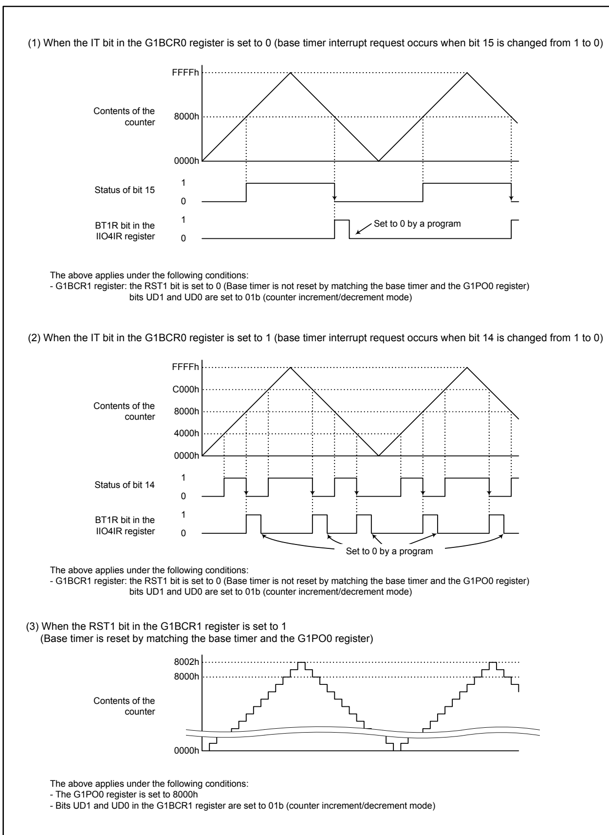
Figure 22.17 Base Timer Operation in Count Increment/Decrement Mode (Group 1)
