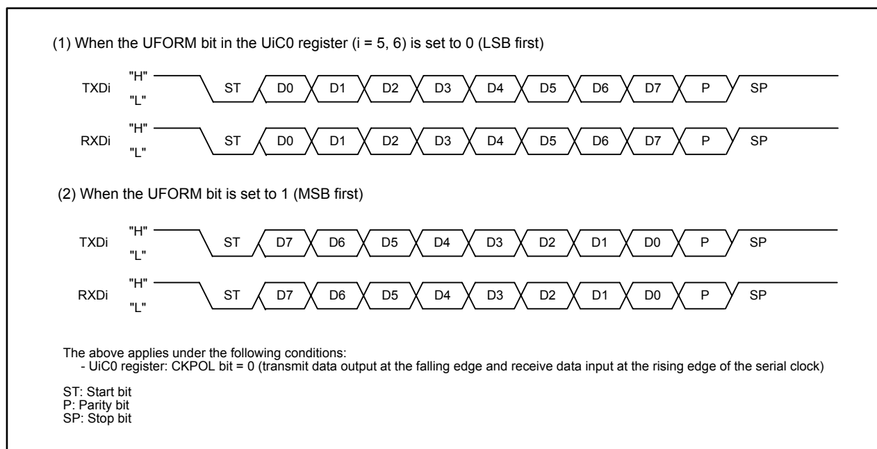
Figure 17.54 Bit Order
