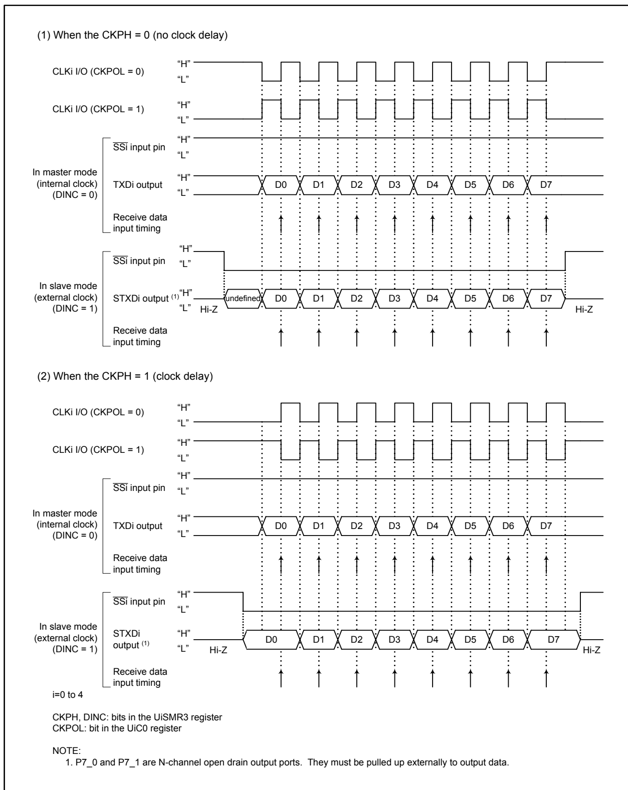
Figure 17.29 Transmit and Receive Operation Timing in Special Mode 2
