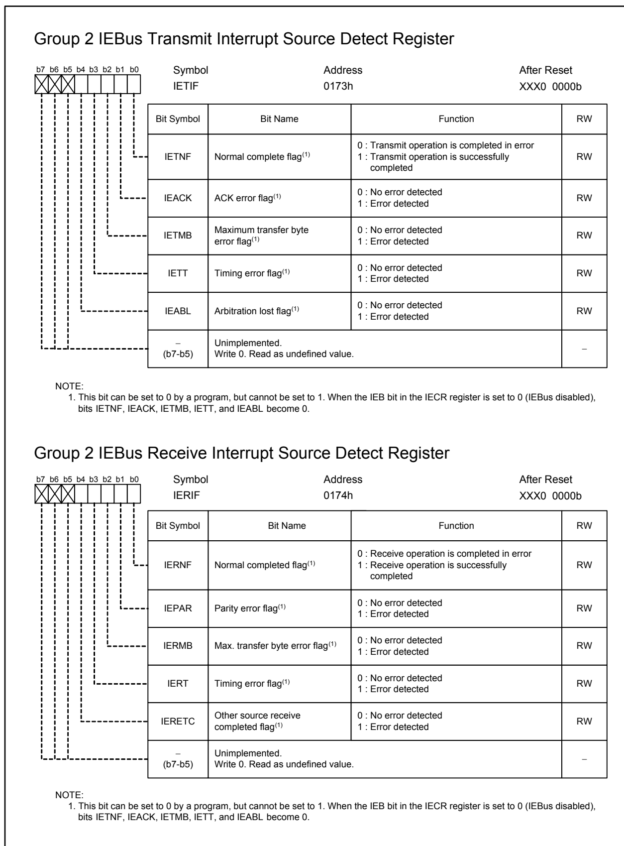
Figure 22.60 IETIF and IERIF Registers
