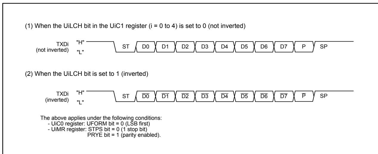
Figure 17.21 Serial Data Logic Inverse
