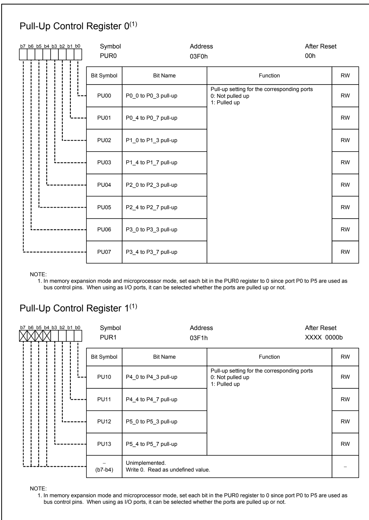
Figure 25.20 PUR0 Register, PUR1 Register
