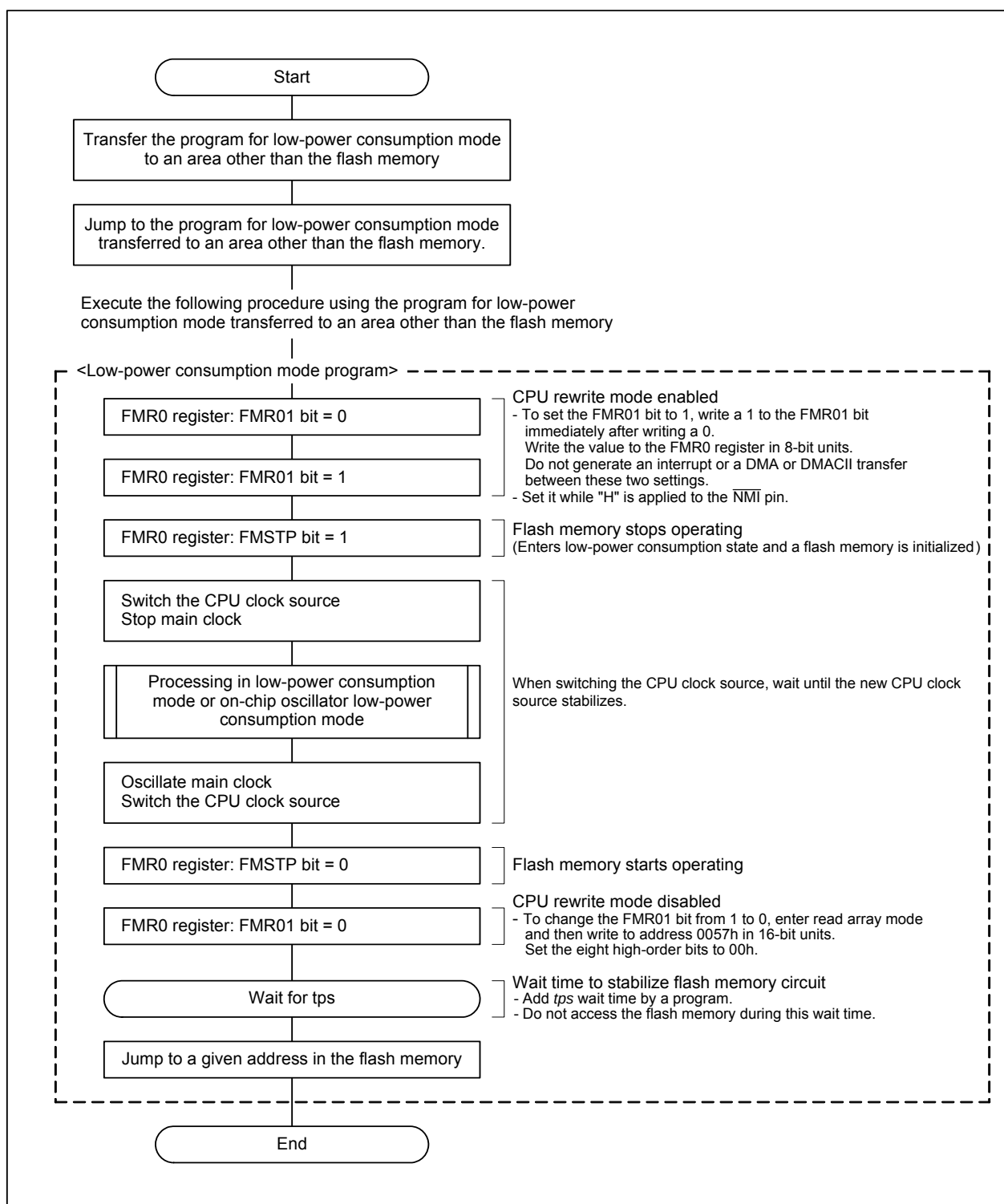
Figure 26.8 Setting Procedure to Enter and Exit Low Power Mode
