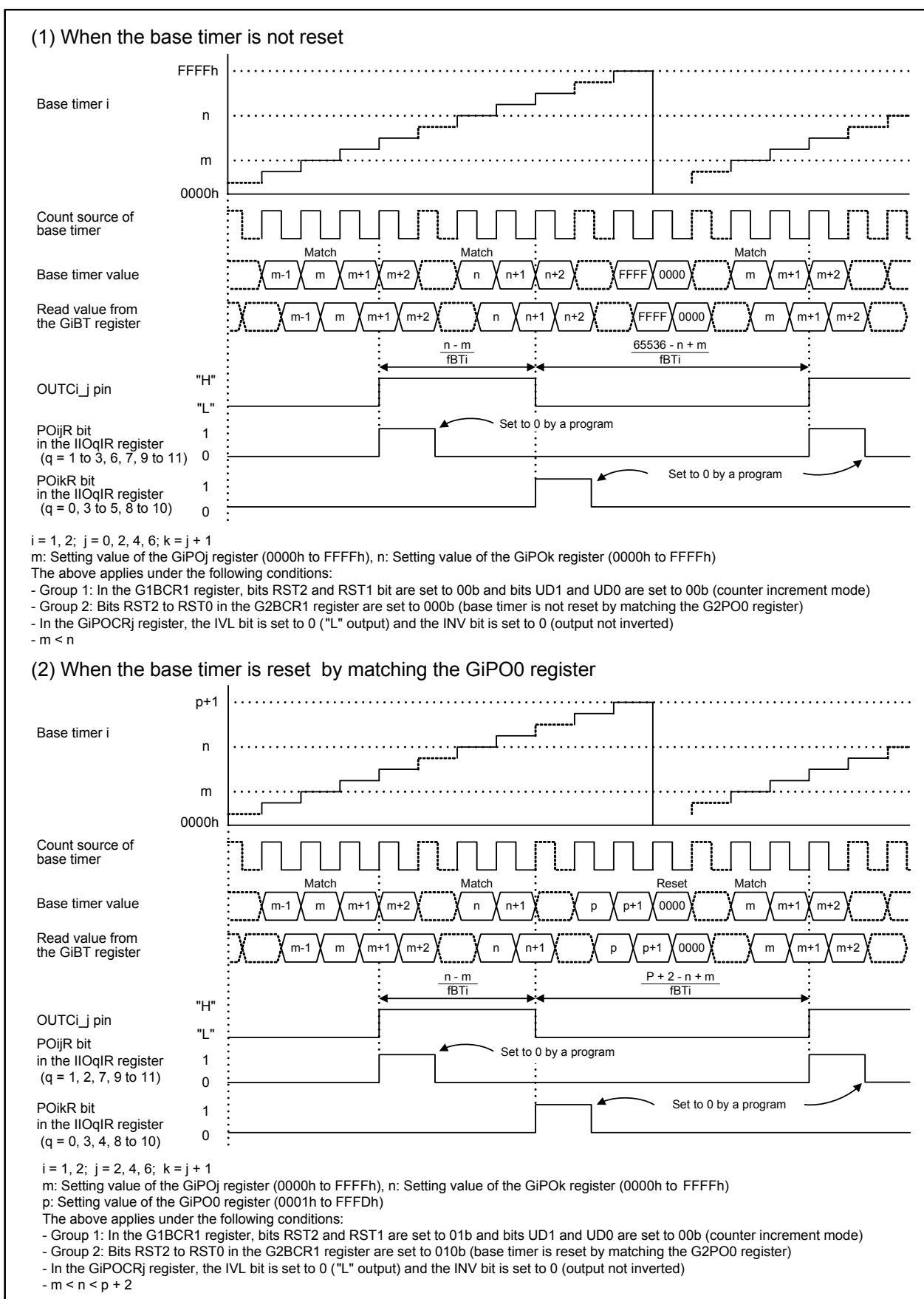
Figure 22.29 SR Waveform Output Mode Operation
