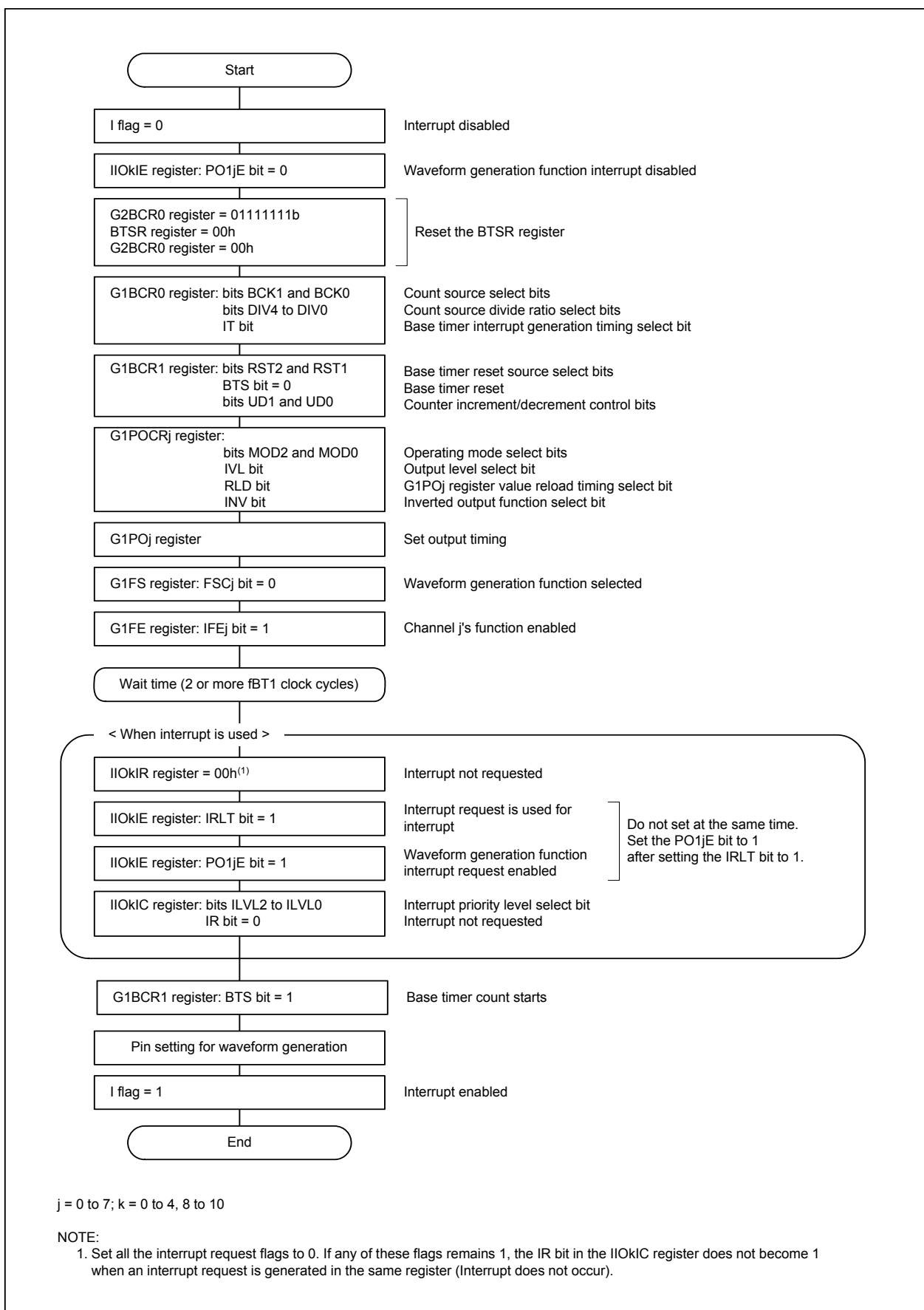
Figure 22.25 Register Settings for Waveform Generation Function (Group 1)
