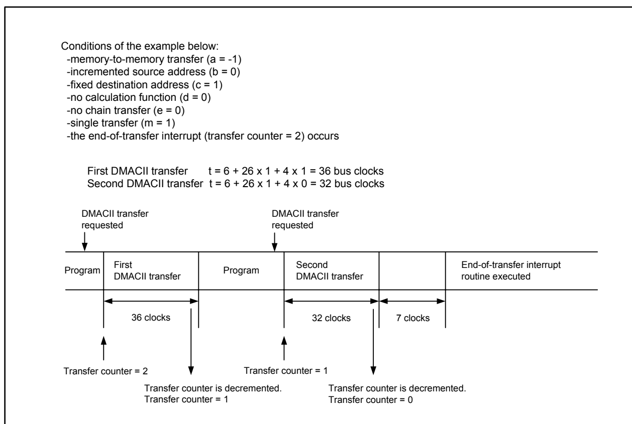
Figure 14.5 Transfer Time
