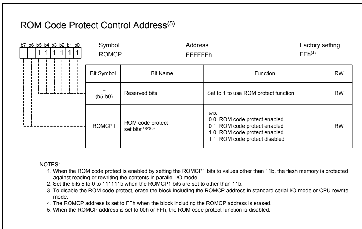
Figure 26.2 ROMCP Address
