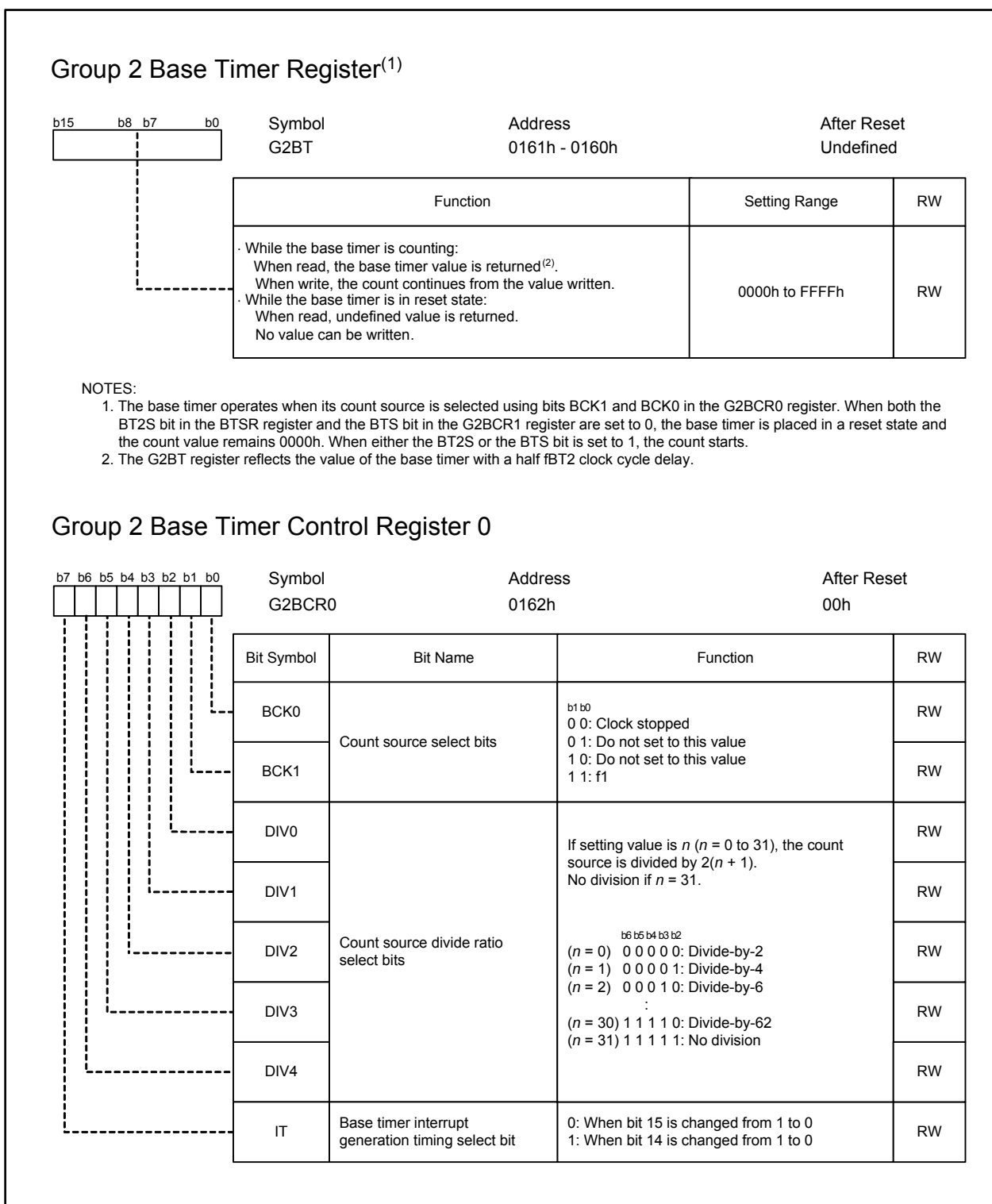
Figure 22.9 G2BT Register, G2BCR0 Register
