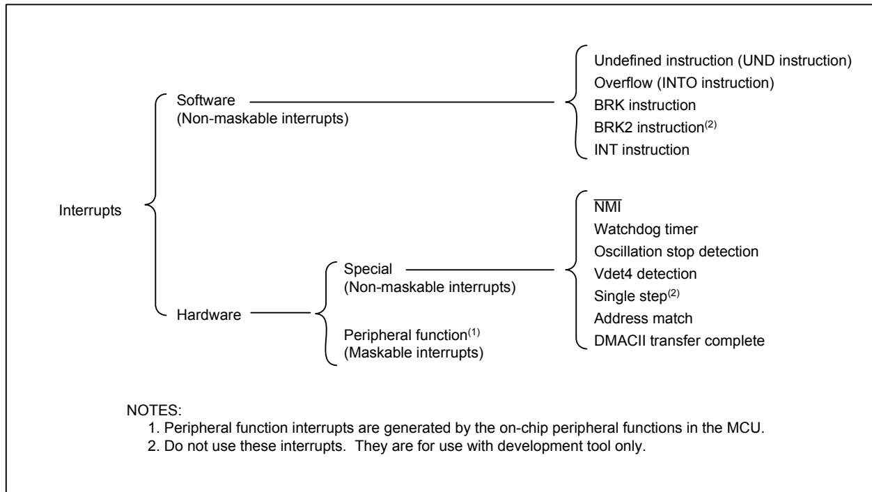
Figure 11.1 Interrupts
