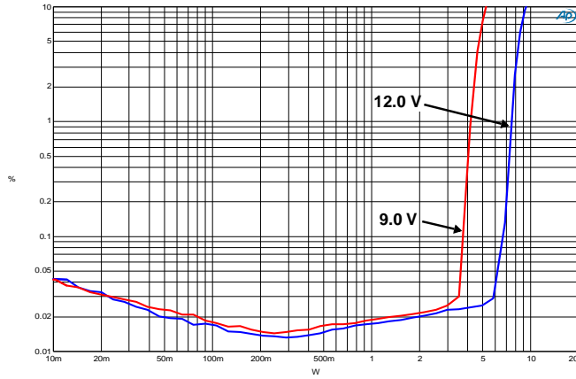
Figure 5. THD+N vs. Output Power ( R_L = 8 \Omega )
