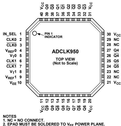
Figure 2. Pin Configuration
