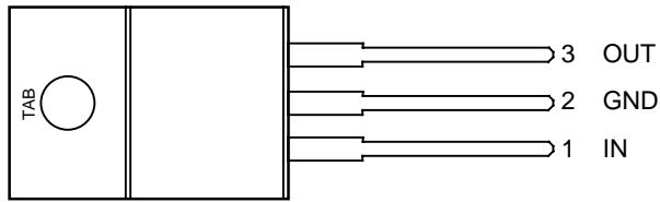
MIC29310-x.xBT TO-220 (T)
