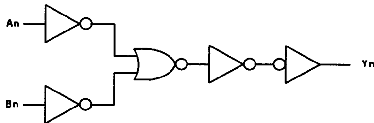
FIGURE 3. Logic diagram.
