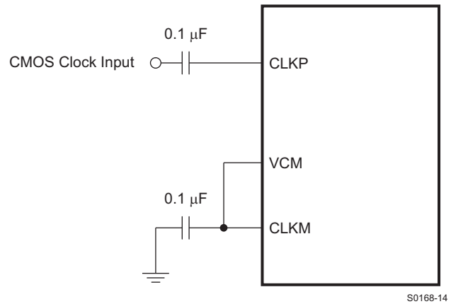
Figure 103. Single-Ended Clock Driving Circuit
