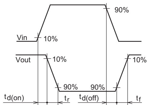
Waveforms
