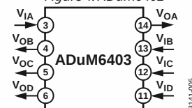
Figure 5. ADuM6403
