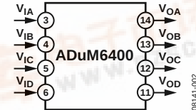
Figure 2. ADuM6400
