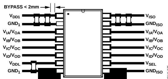
Figure 25. Recommended Printed Circuit Board Layout
