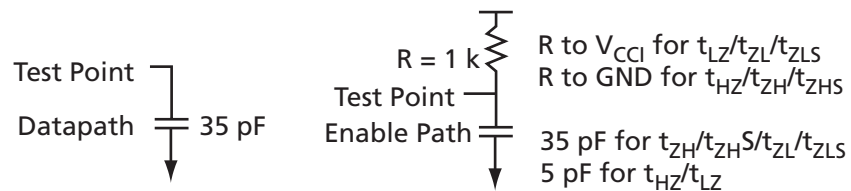
Figure 2-6 • AC Loading
