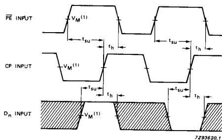
Fig. 10 Waveforms showing the set-up and hold times for the input ( D_n ) and parallel enable input (PE).
