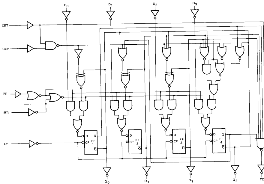
Fig. 7 Logic diagram.
