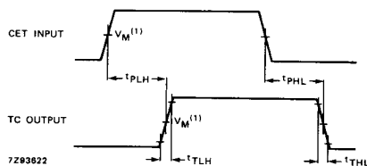
Fig. 9 Waveforms showing the input (CET) to output (TC) propagation delays and output transition times.
