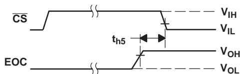
Figure 31. \overline{CS} and EOC Waveforms
