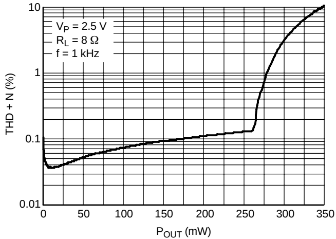
Figure 2. THD+N versus Output Power
