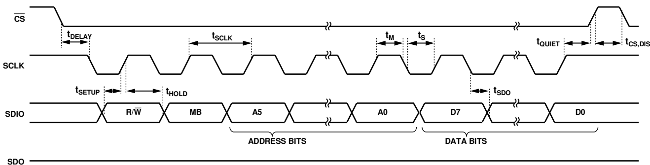
Figure 31. SPI 3-Wire Read/Write
