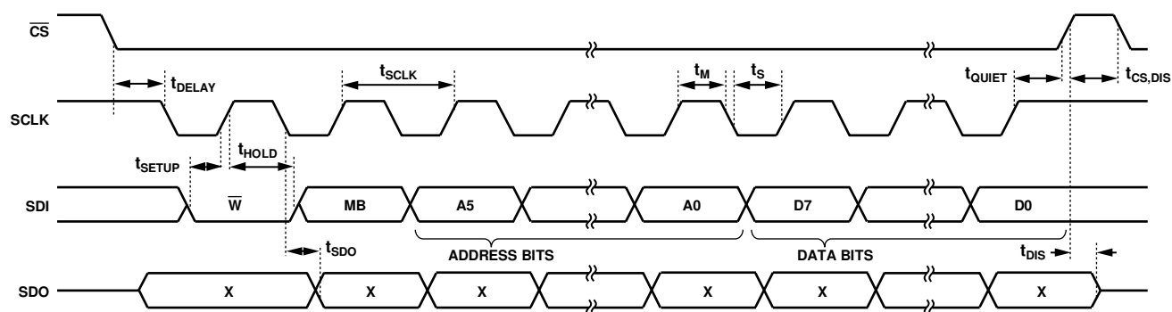
Figure 29. SPI 4-Wire Write
