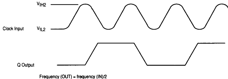
Figure 1. FMAX Test Circuit and Clock Input Sinewave
