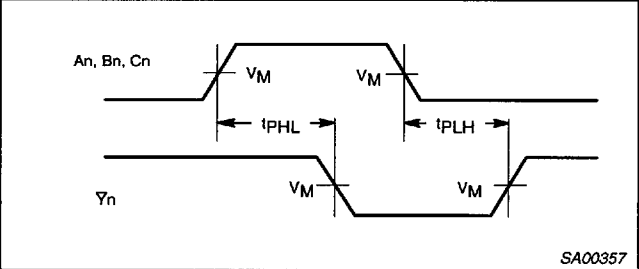
Waveform 1. Propagation Delay for Inverting Outputs
