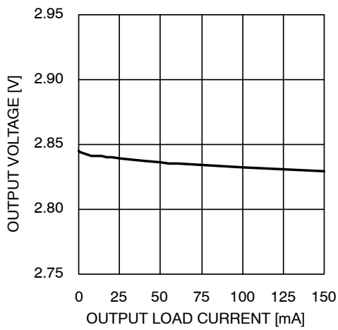
Figure 5. Load Regulation
