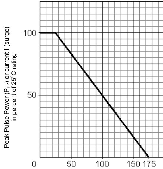
FIG. 4 Derating Curve
