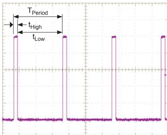
V CC at Various Duty Cycles 4 \mu s per division
