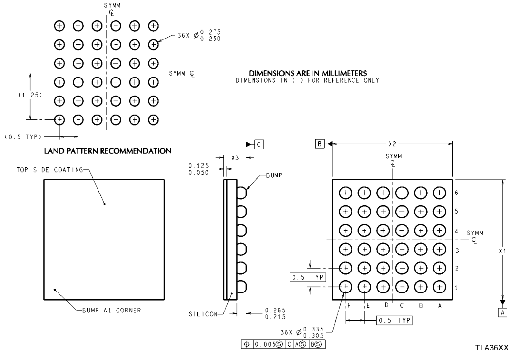
36-Bump uSMD Package NS Package Number TLA36TTA
