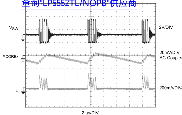
V COREx Burst-PWM Switching Waveform 查询"LP5552TL/NOPB"供应商
