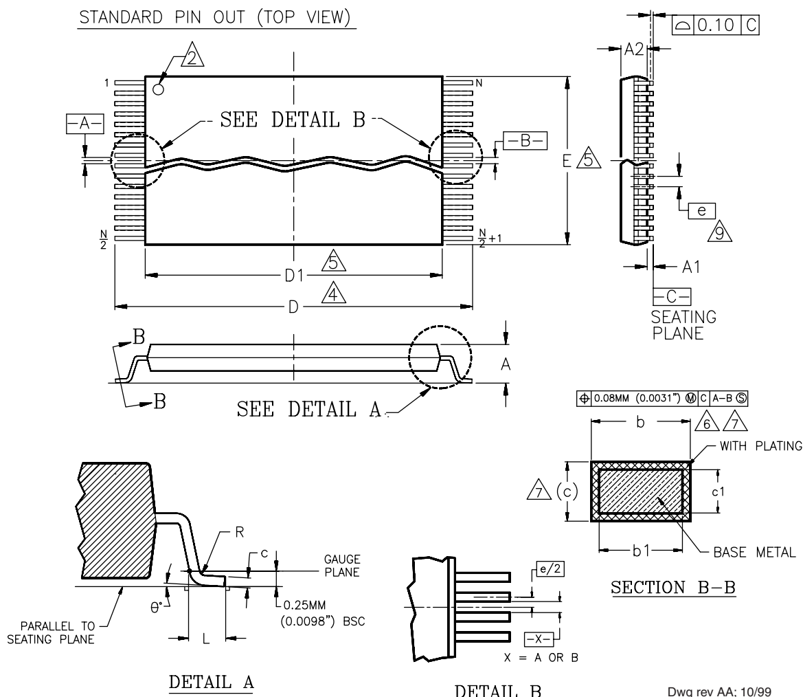
DETAIL B
