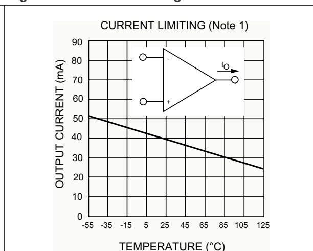
Figure 9. Current limiting
