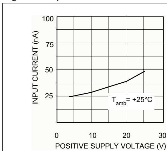
Figure 14. Input current
