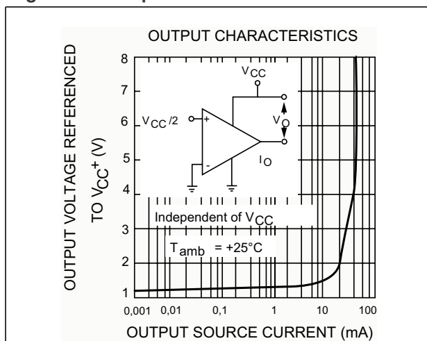
Figure 8. Output characteristics
