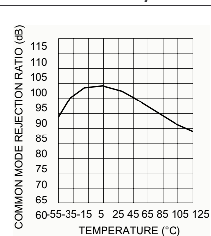
Figure 17. Common mode rejection ratio
