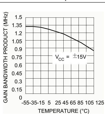
Figure 15. Gain bandwidth product
