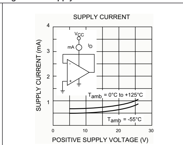
Figure 13. Supply current
