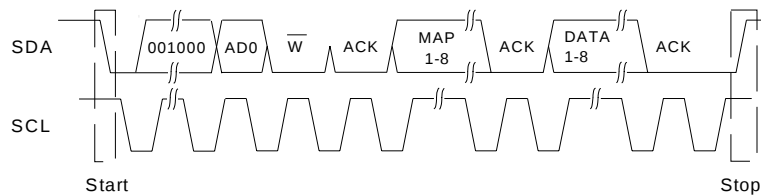
Figure 22. I²C Write
