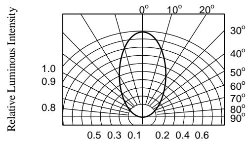
FIG.6 RADIATION DIAGRAM
