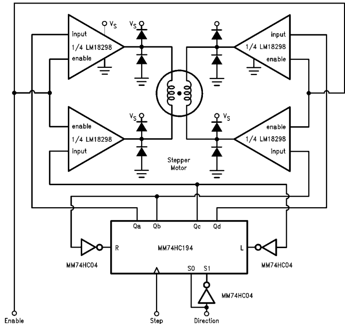
FIGURE 6. Two-Phase Bipolar Stepper Motor Control Circuit
