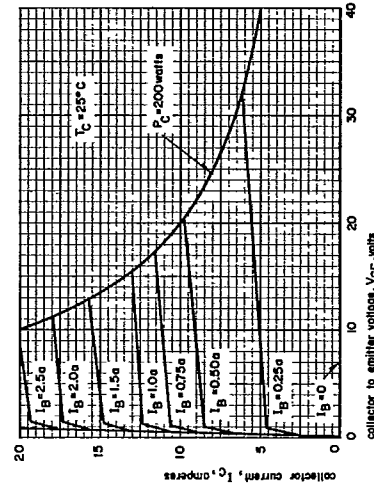
figure 2. Output characteristics.
