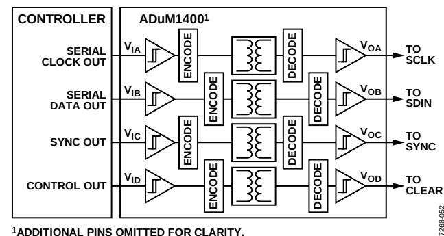
Figure 58. Isolated Interface
