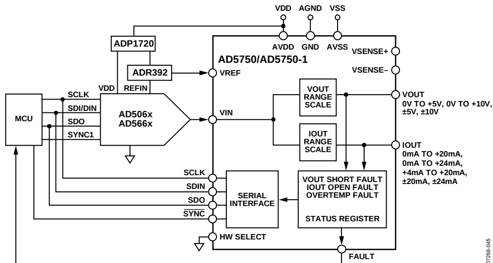
Figure 51. Typical System Configuration in Software Mode (Pull-Up Resistors Not Shown for Open-Drain Outputs)
