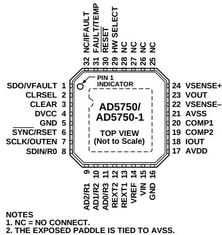
Figure 4. Pin Configuration
