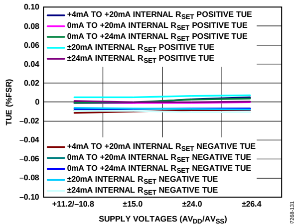
Figure 31. Total Unadjusted Error Current Mode, Internal R_{SET} Sense Resistor
