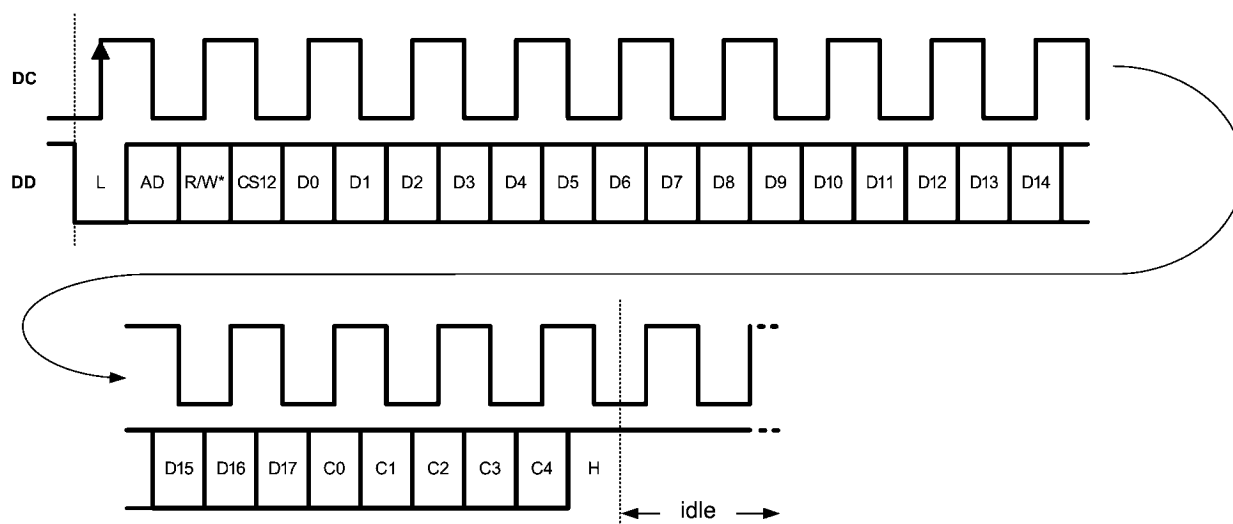
FIGURE 8. WRITE Transaction
