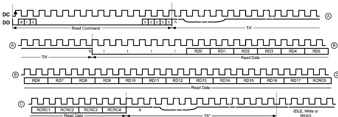
FIGURE 10. READ Transaction
