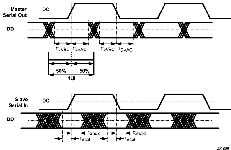
FIGURE 1. Serial Data Valid & Set/Hold Times
