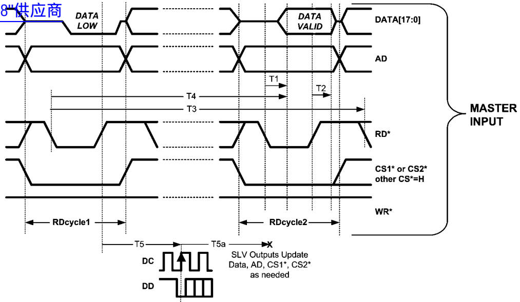
FIGURE 11. Master Input READ Timing
