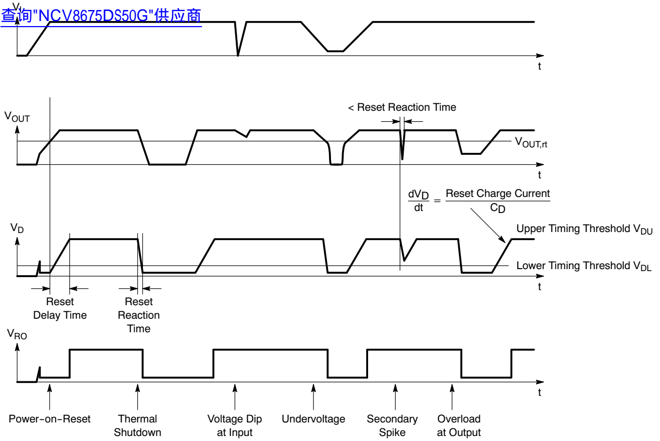
Figure 35. Reset Timing
