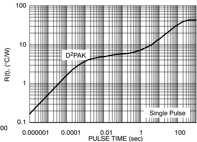
Figure 38. NCV8675 @ PCB Cu Area 100 mm² PCB Cu thk 1 oz
