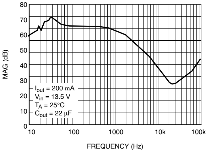
Figure 14. Power Supply Rejection Ratio (5 V Version)
