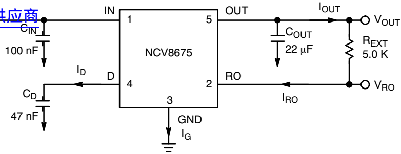
Figure 34. Application Circuits
