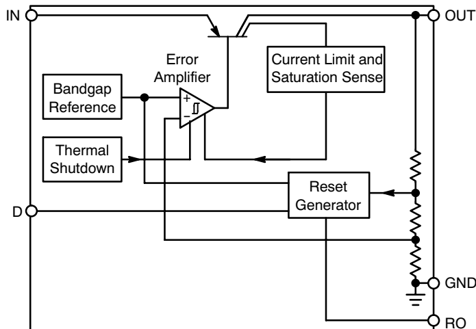
Figure 1. Block Diagram
