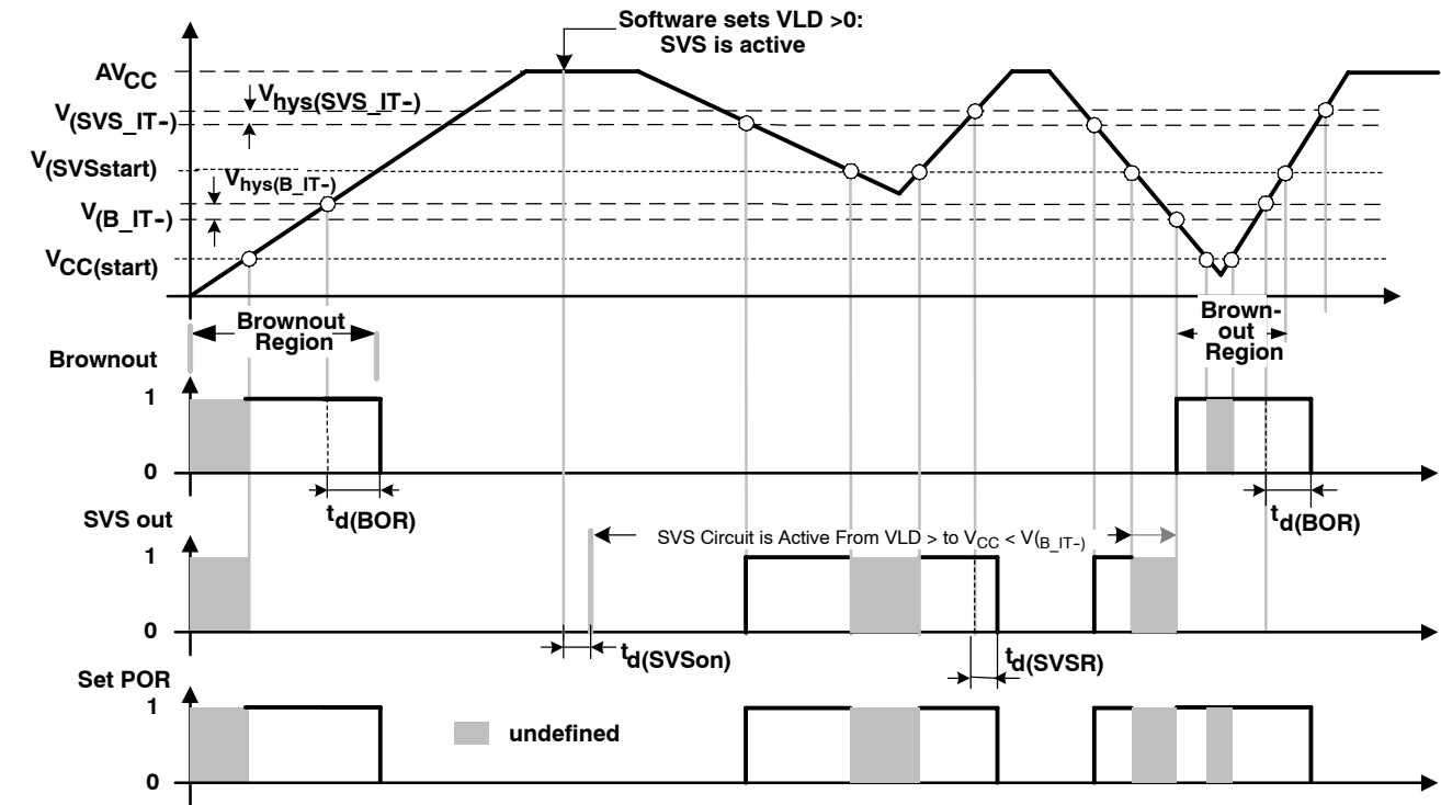
Figure 12. SVS Reset (SVSR) vs Supply Voltage
