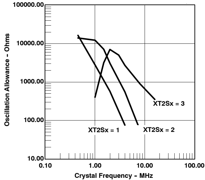
Figure 25. Oscillation Allowance vs Crystal Frequency, C_{L,eff} = 15 \text{ pF} , T_A = 25^\circ\text{C}
