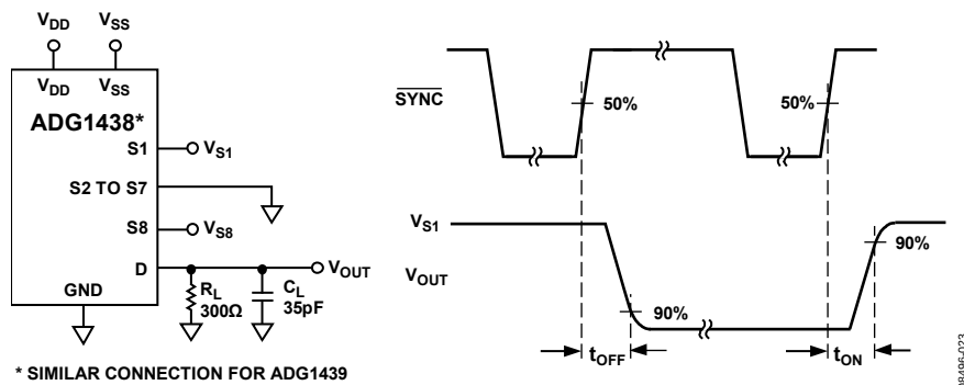
Figure 30. Switching Times, t_{ON}/t_{OFF}
