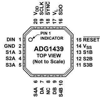
Figure 8. ADG1439 Pin Configuration (LFCSP)
