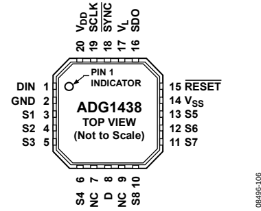
Figure 6. ADG1438 Pin Configuration (LFCSP)
