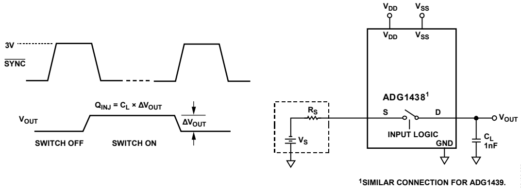
Figure 32. Charge Injection
