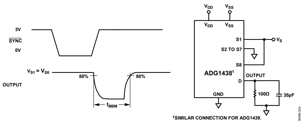
Figure 31. Break-Before-Make Delay, t_{BBM}
