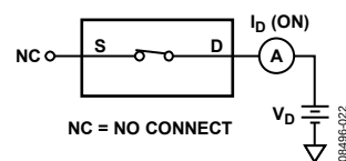
Figure 29. On Leakage
