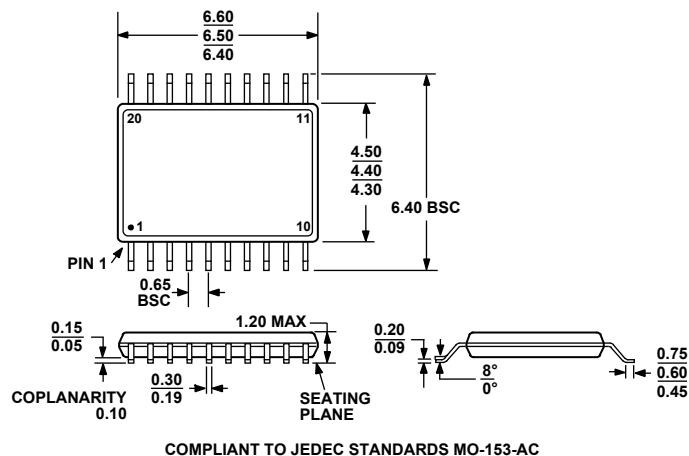
Figure 37. 20-Lead Thin Shrink Small Outline Package [TSSOP] (RU-20)
