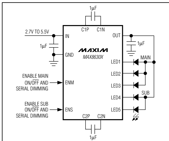
Figure 1. Typical Applications Circuit with the MAX8630X
