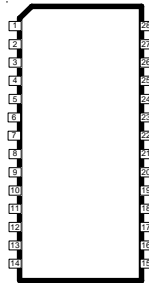
A3940KLW (SOIC)
