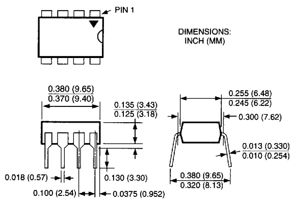
8-Pin Plastic DIP (N)
