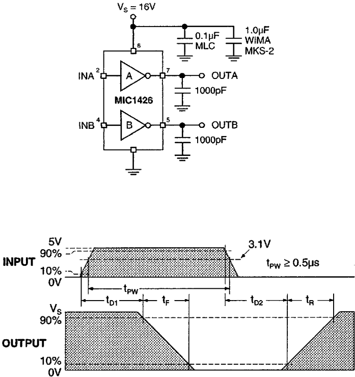
Figure 1. Inverting Driver Switching Time
