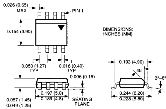
8-Pin SOIC (M)
