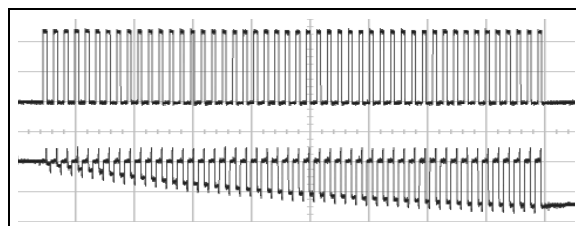
Figure 2-3 Vcs - Correct
