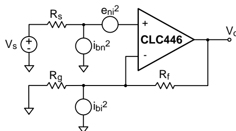
Figure 9: Noise Model
