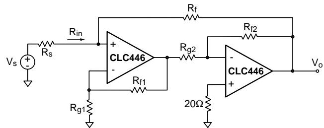
Figure 10: Composite Amplifier
