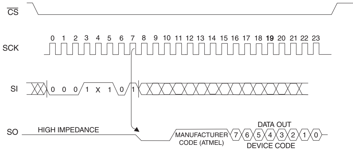
Figure 13. RDID Timing
