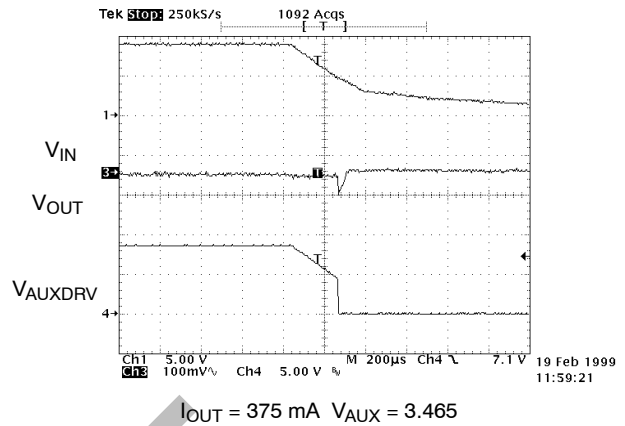
Figure 19. Power-Down, V_{AUX} = 3.465 \text{ V}
