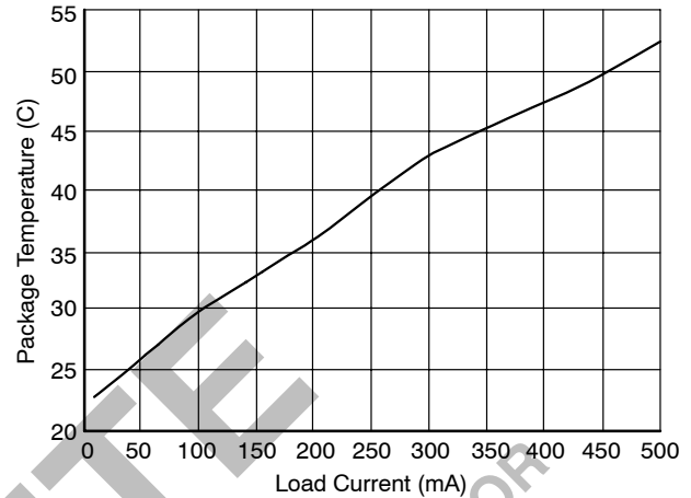
Figure 25. Package Temperature vs. Load Current ( V_{IN} = 5.0 V, T_A = 23^\circ\text{C} )
