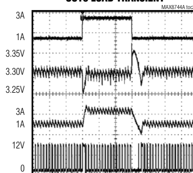
OUT3 LOAD TRANSIENT
