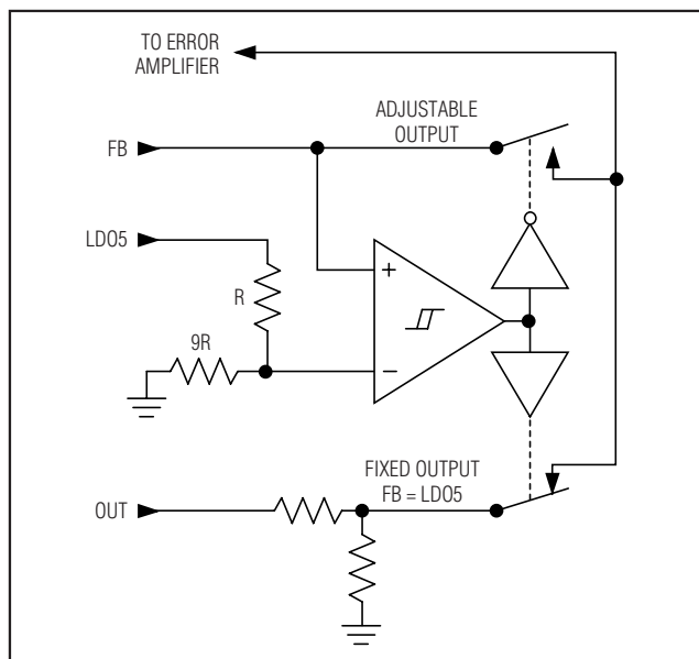
Figure 5. Dual Mode Feedback Decoder
