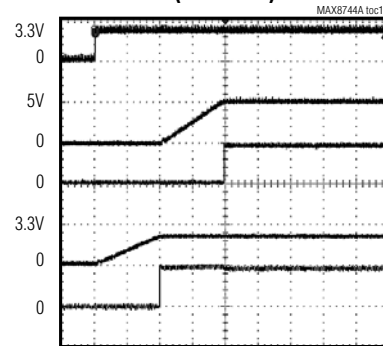
SMPS DELAYED STARTUP SEQUENCE (ON5 = REF)
