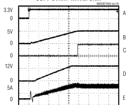
SOFT-START WAVEFORM
