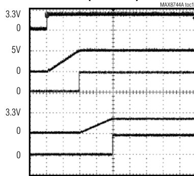
SMPS DELAYED STARTUP SEQUENCE (ON3 = REF)
