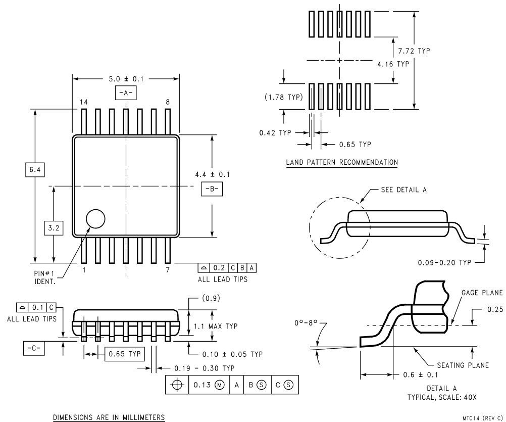
14-Pin TSSOP NS Package Number MTC14
