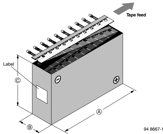
Figure 21. Tape Direction
